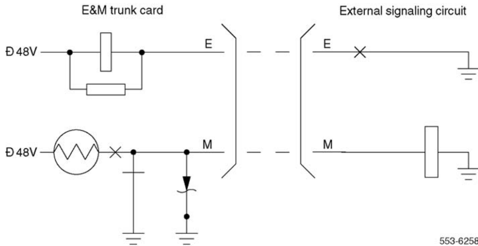
Figure 140: E and M Type I signaling
