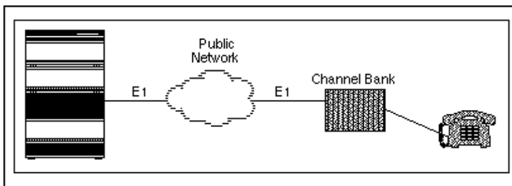
Figure 71: LEI in off-premise extension application
