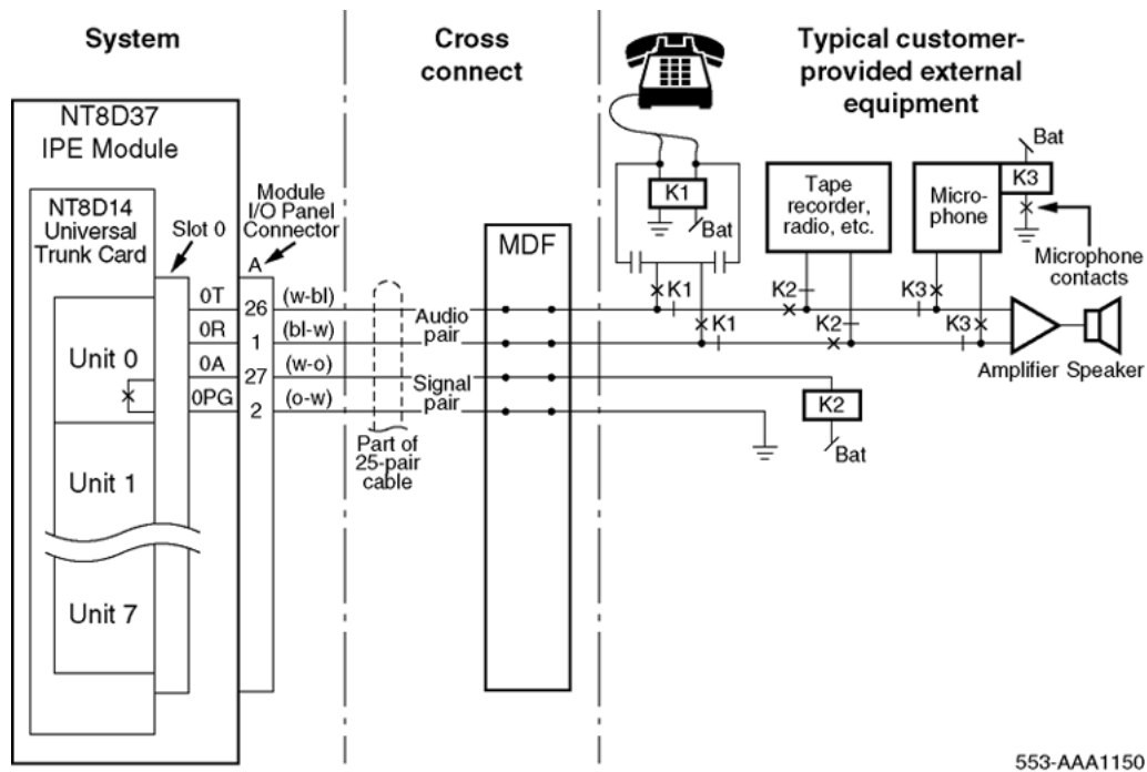
Figure 152: Paging trunk operation
