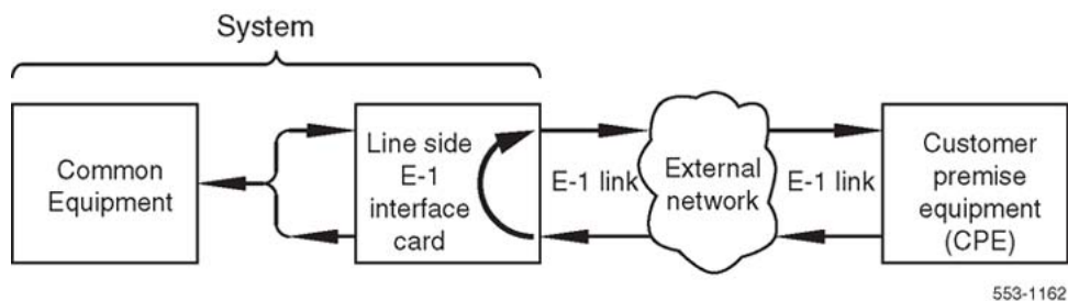
Figure 69: MMI Network loopback test
