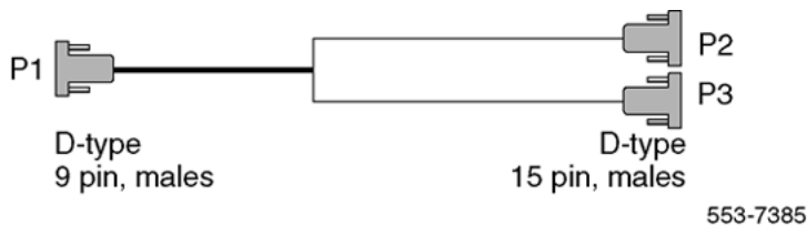
Figure 76: NTCK78AA
