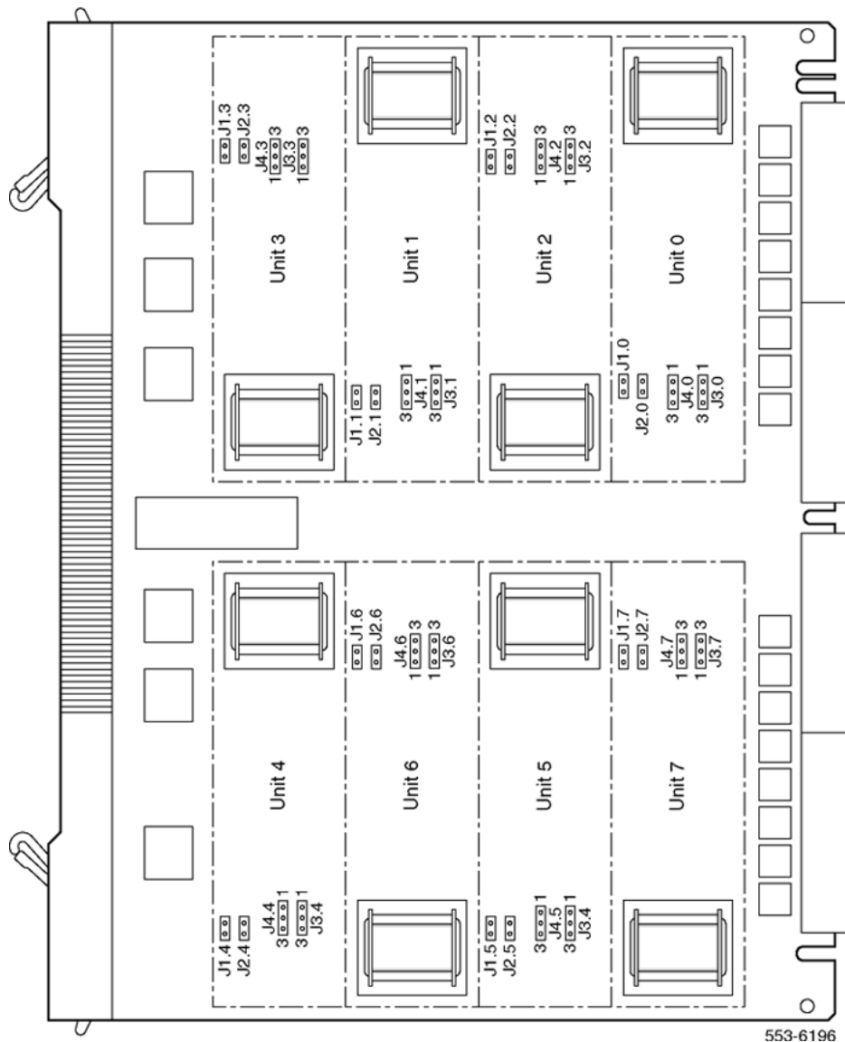
Figure 135: Universal trunk card - jumper locations for NT8D14BA and NT8D14BB Release 9 and below
