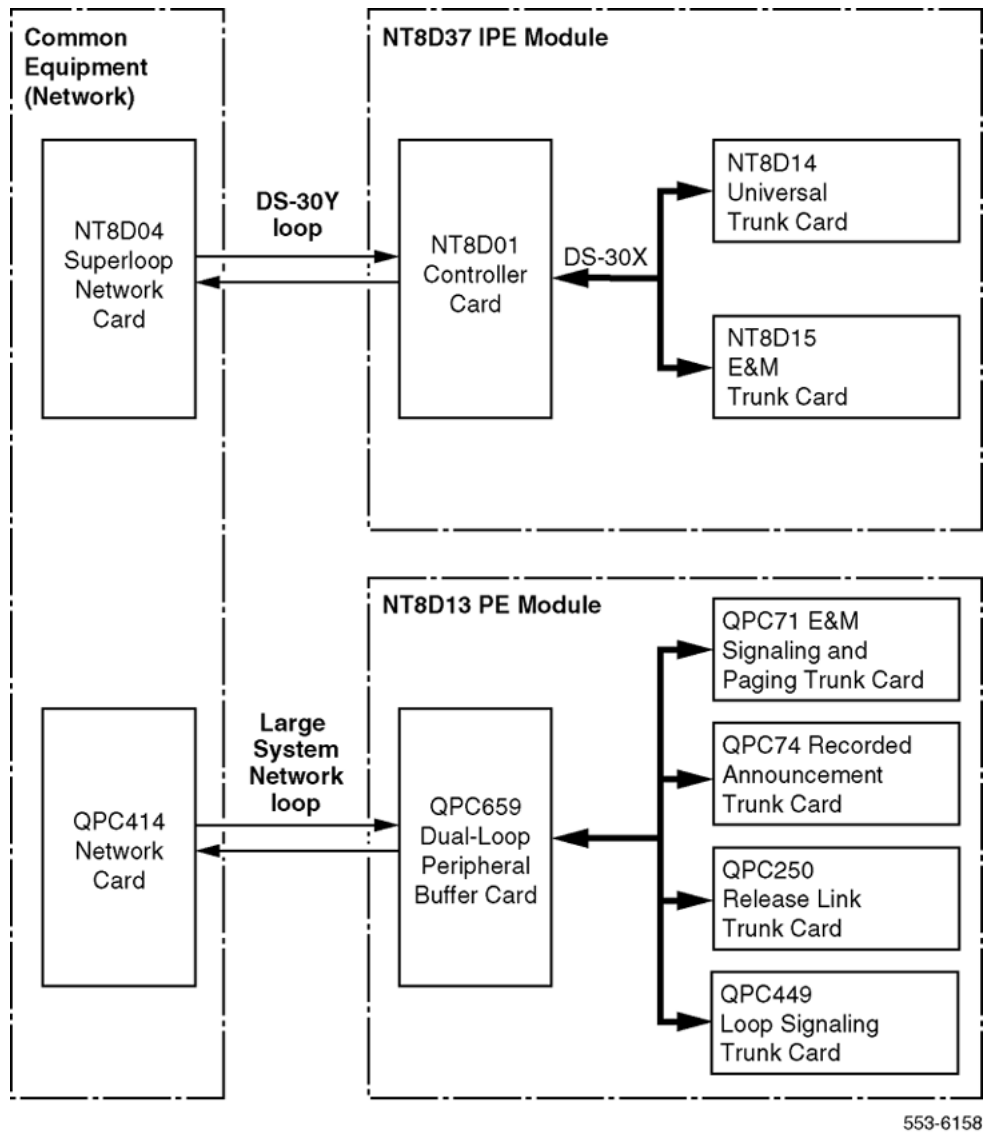
Figure 15: Network connections to IPE modules
