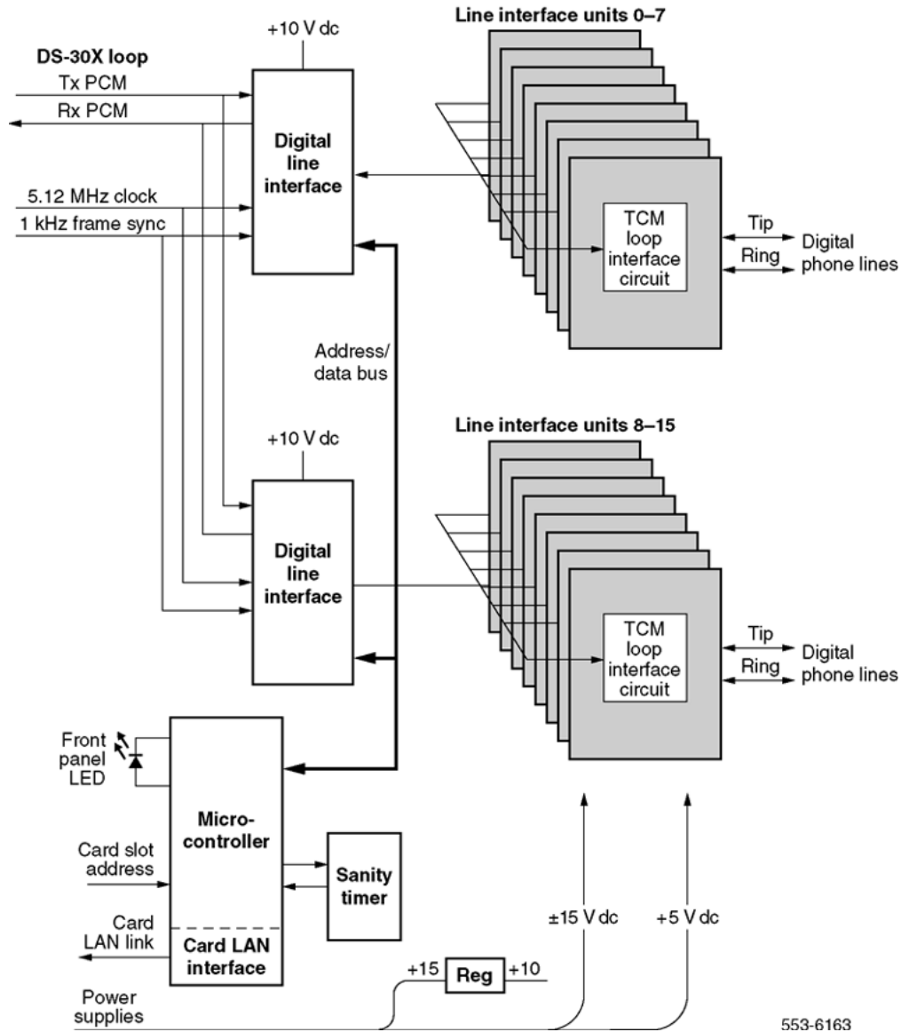
Figure 103: Digital line card - block diagram
