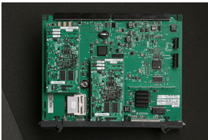
Figure 191: Media Gateway Controller with daughterboards
