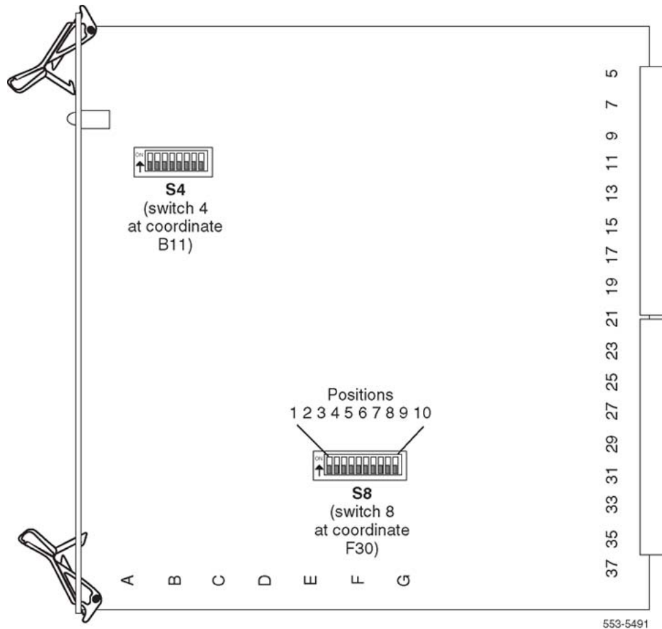
Figure 19: Circuit card grid
