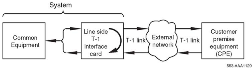
Figure 38: MMI local loopback test
