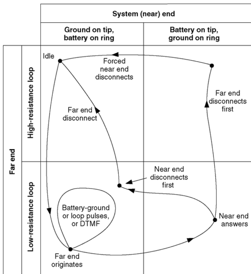
Figure 129: Two-way, loop OAID, TIE trunk call states - incoming call from far-end PBX
