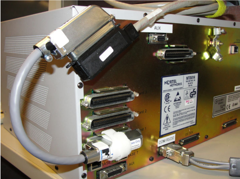
Figure 12: Connecting the surge suppression cable to the CS 1000 system MDF cable
