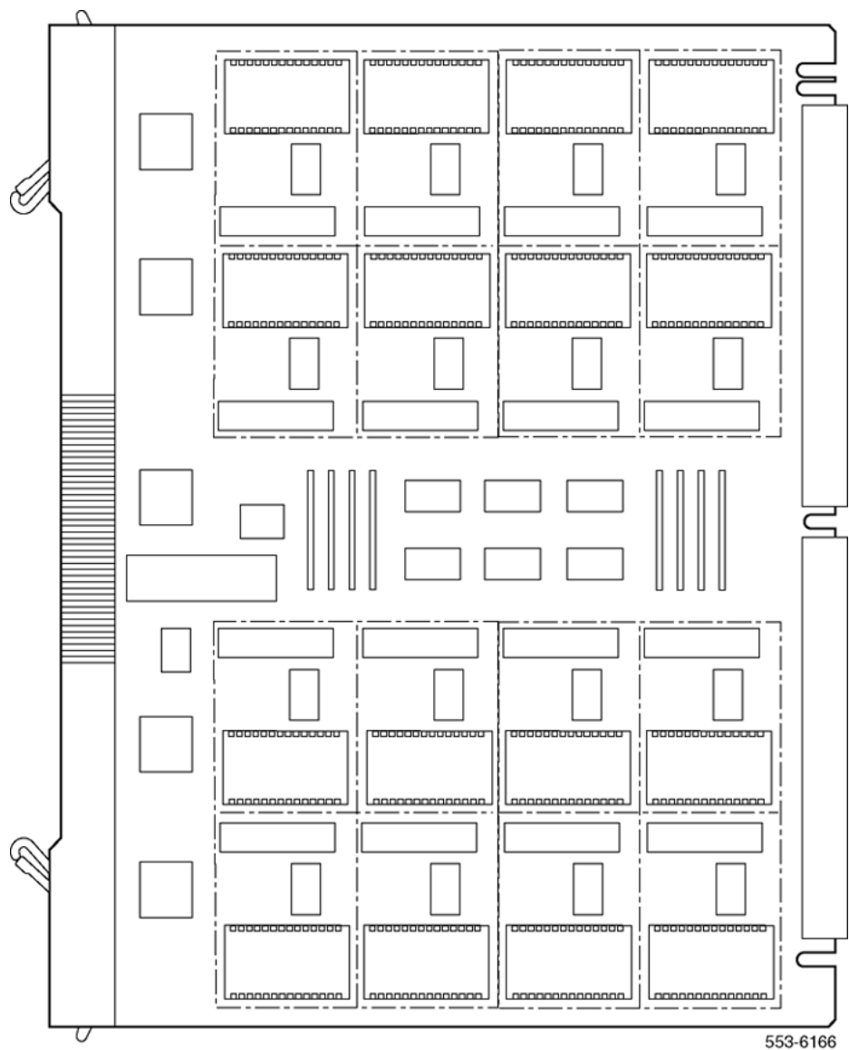
Figure 108: Analog message waiting line card - jumper block and switch locations
