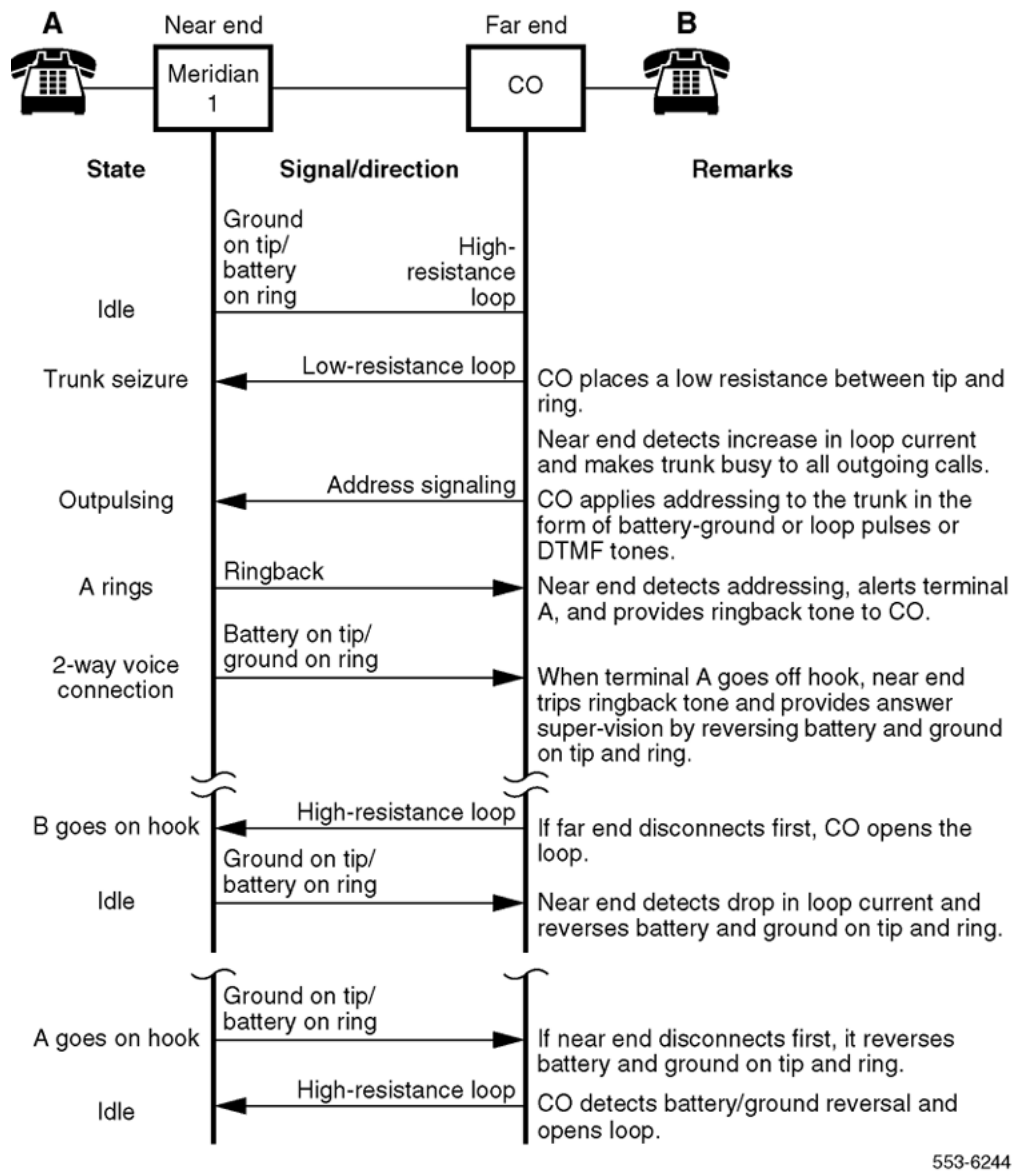
Figure 125: Two-way, loop DR, TIE trunk call states - outgoing call to far-end PBX
