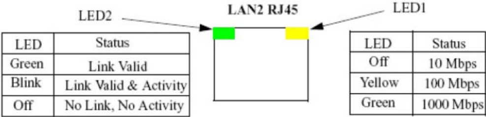
Figure 190: HSP port LED indicators
