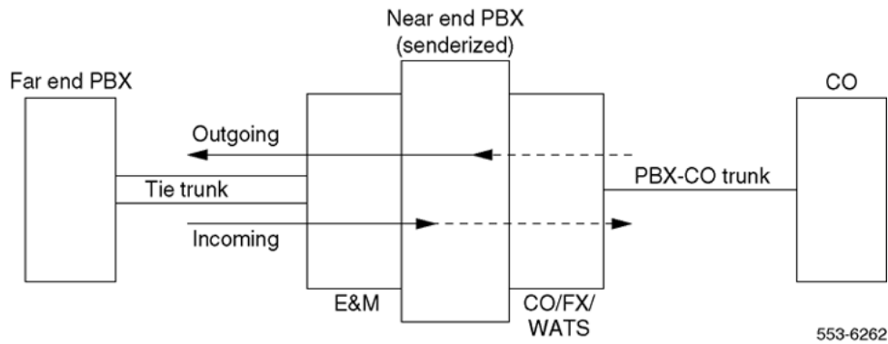
Figure 144: Signaling orientation for tandem connection between E and M and CO trunks
