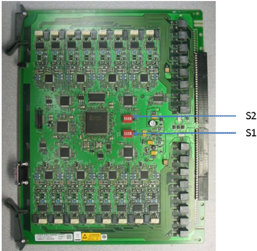
Figure 99: Analog message waiting line card - switch locations
