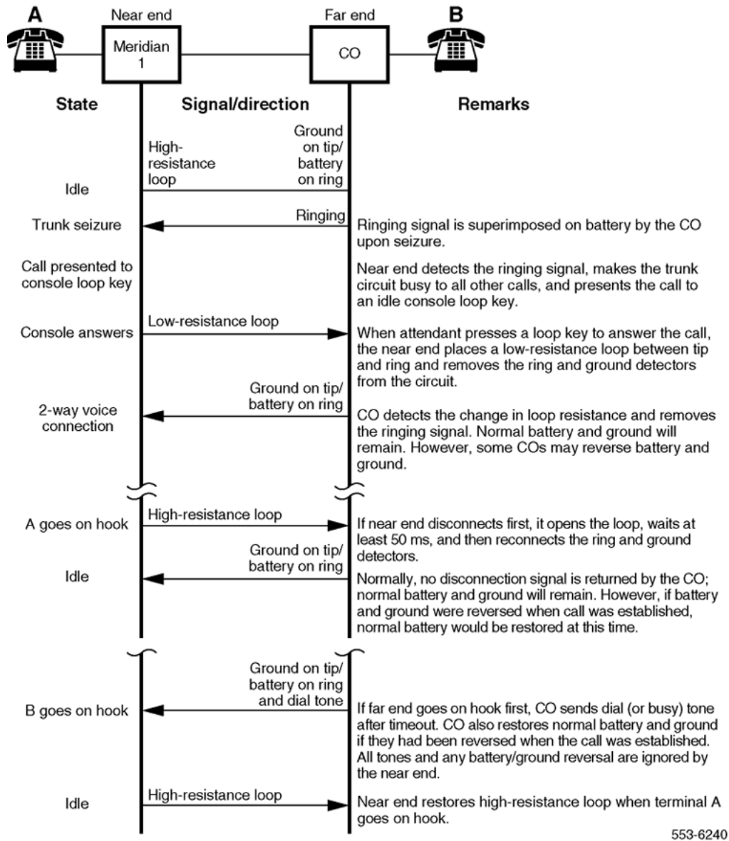
Figure 112: Loop start call connection sequence - incoming call from CO/FX/WATS
