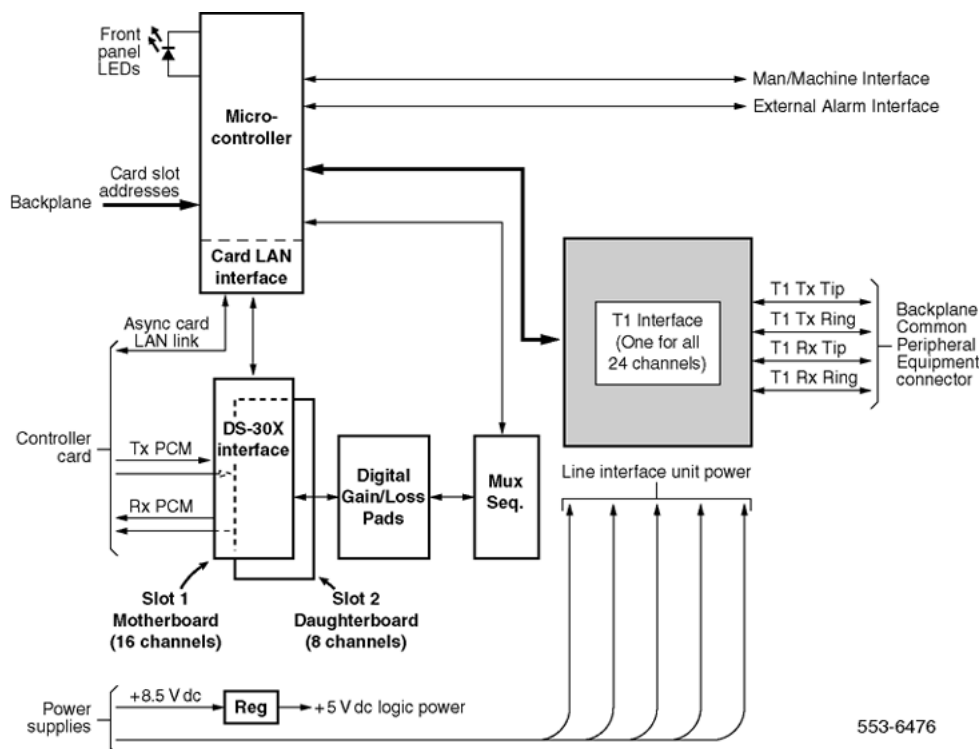
Figure 30: Lineside T1 card - block diagram
