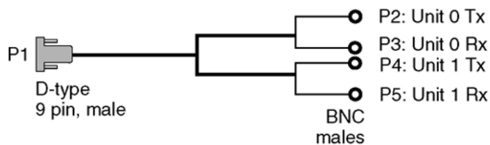
Figure 77: NTCK79AA
