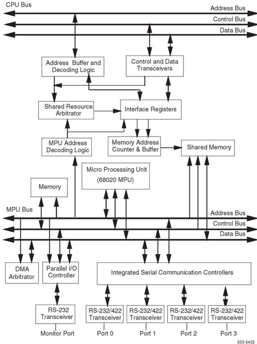
Figure 91: MSDL block diagram
