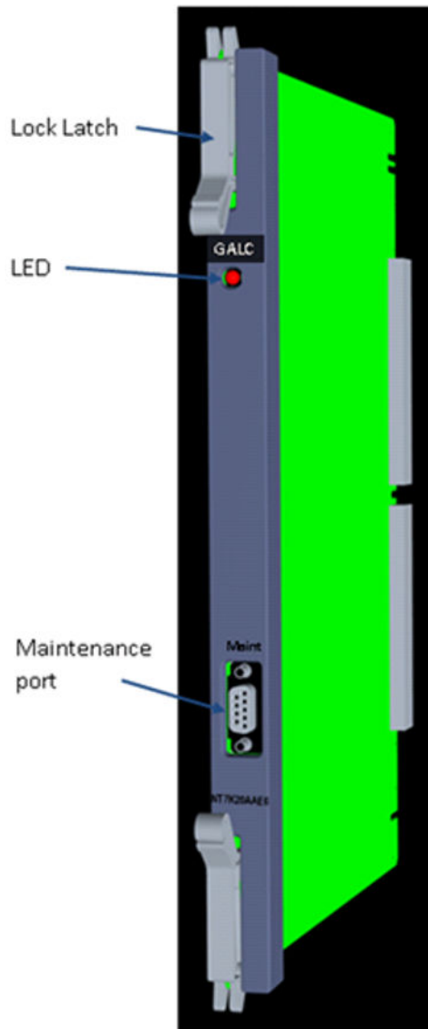
Figure 96: Analog message waiting line card - faceplate
