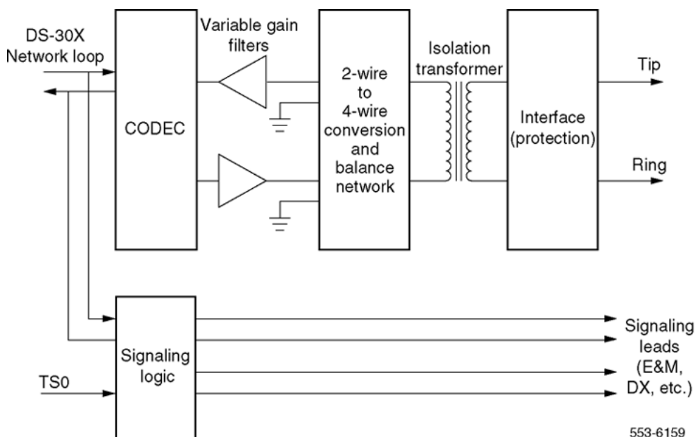
Figure 16: Typical trunk interface unit block diagram
