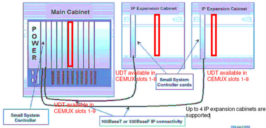
Figure 154: UDT card positioning in Avaya CS 1000M Cabinet/ Meridian 1 PBX 11C Cabinet
