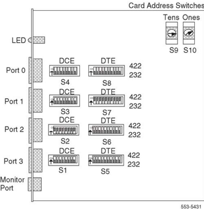
Figure 90: MSDL component layout
