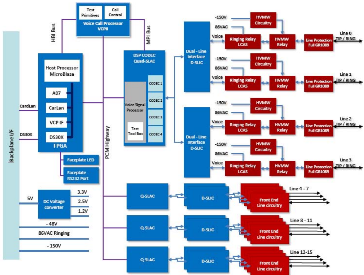
Figure 97: NT7K20- block diagram
