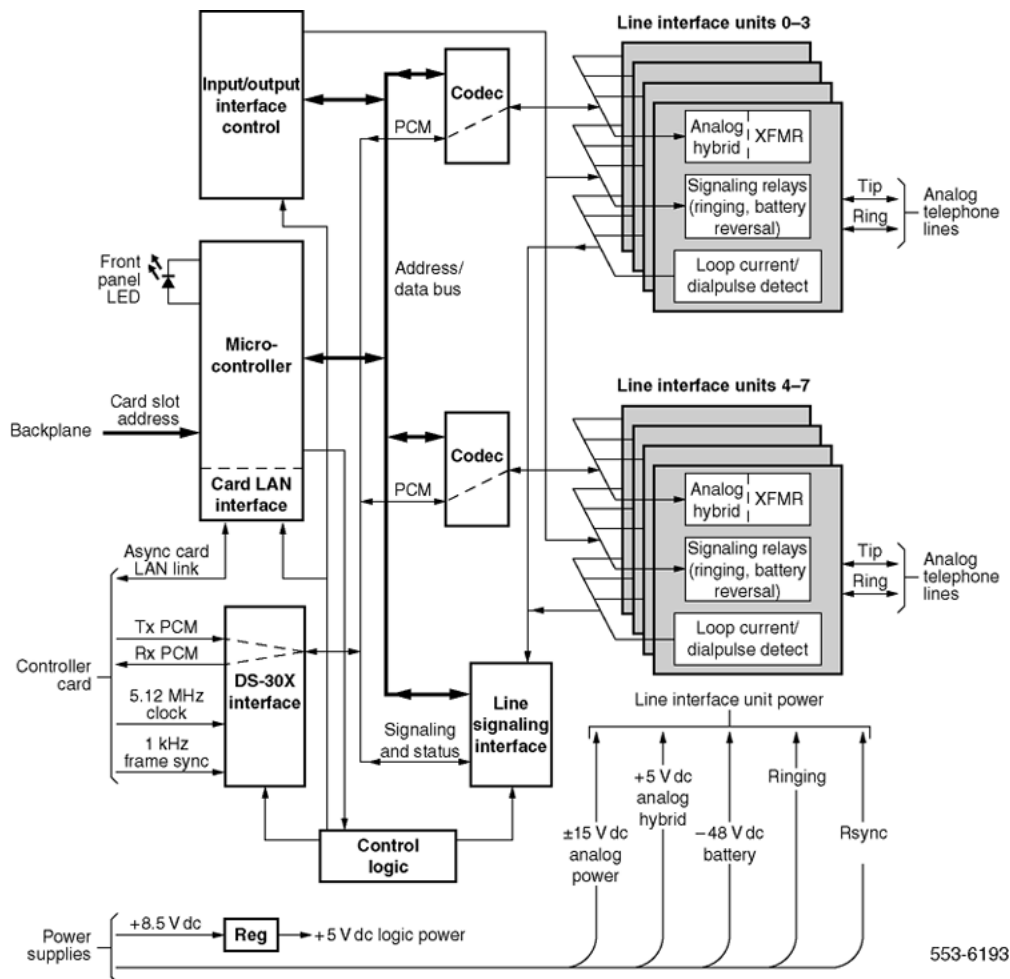
Figure 23: OPS analog line card - block diagram
