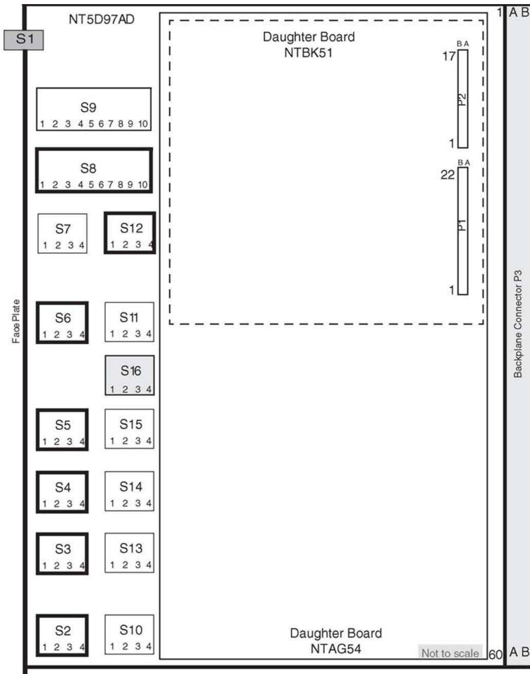
Figure 84: Dip switches locations for NT5D97AD
