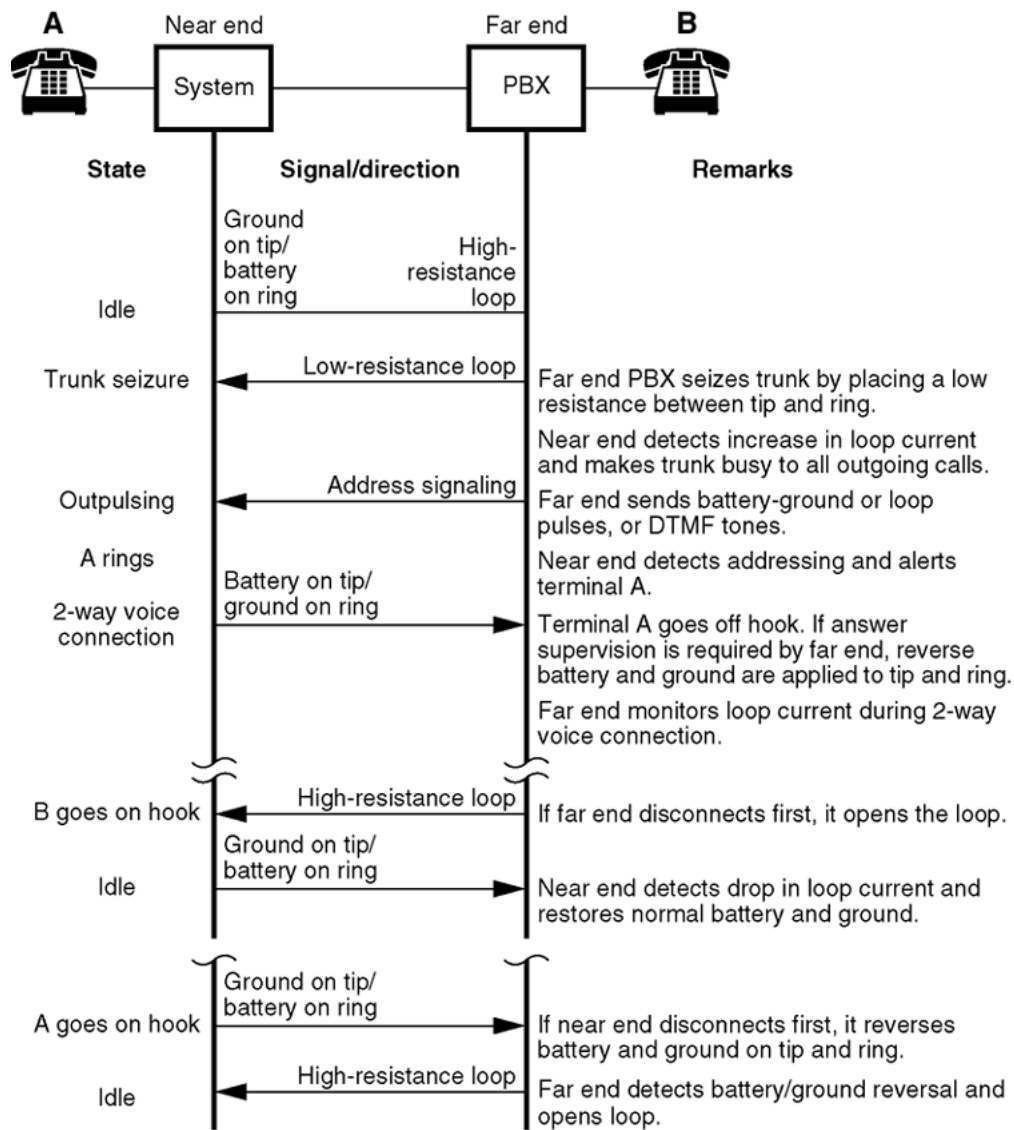
Figure 130: Two-way, loop OAID, TIE trunk call connection sequence - incoming call from far-end PBX
