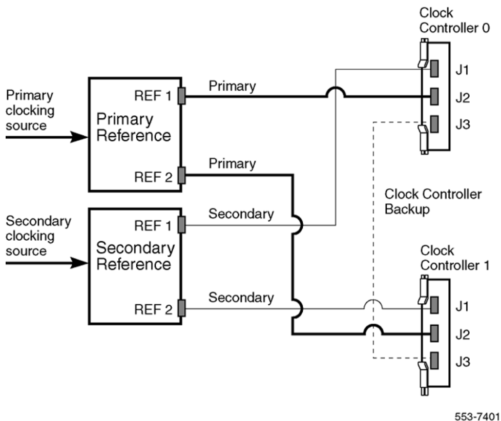
Figure 85: Clock Controller primary and secondary tracking
