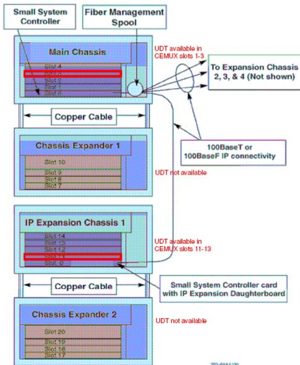
Figure 155: UDT card positioning in CS 1000M Chassis/ Meridian 1 PBX 11C Chassis
