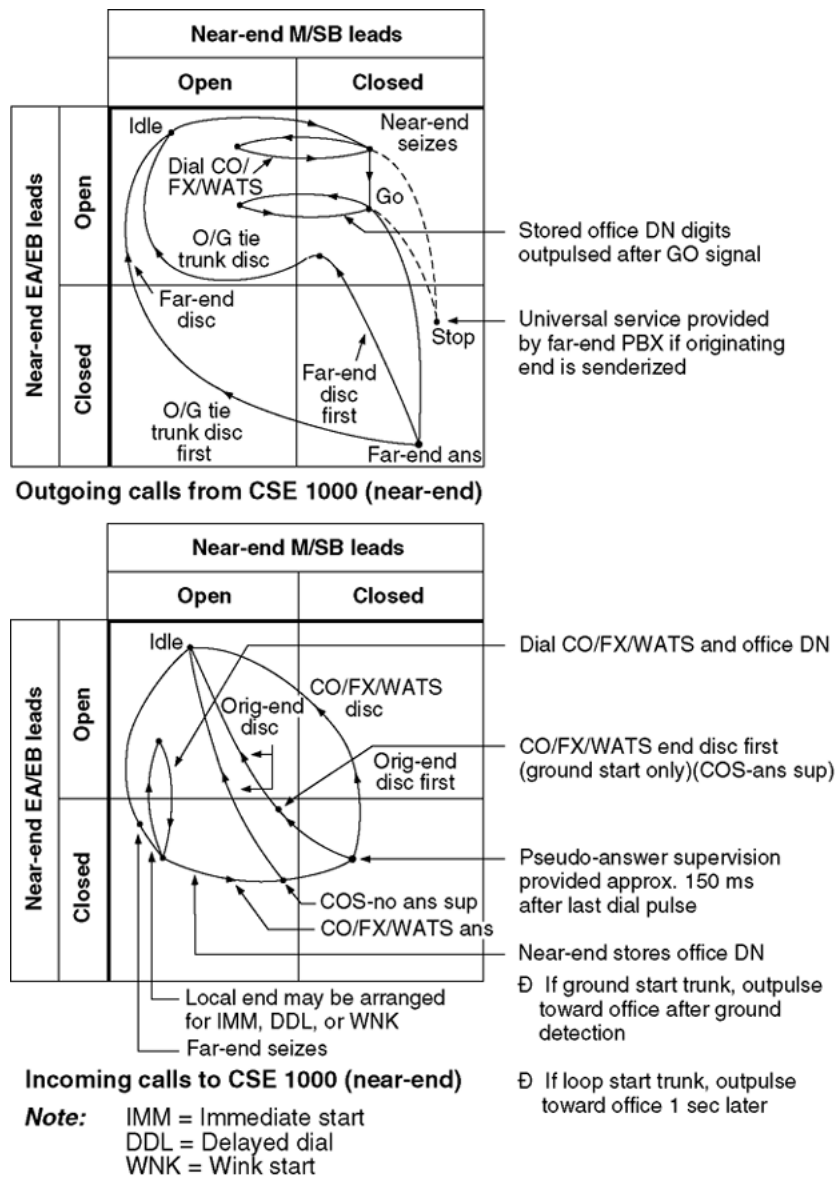
Figure 148: E and M Type II signaling patterns - originating party release on a tandem connection
