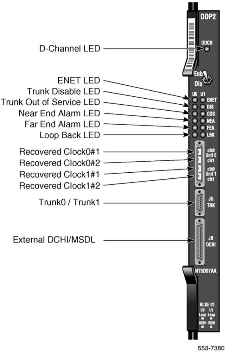
Figure 73: NT5D97 faceplate
