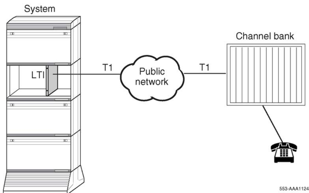
Figure 42: Lineside T1 interface in off-premise application
