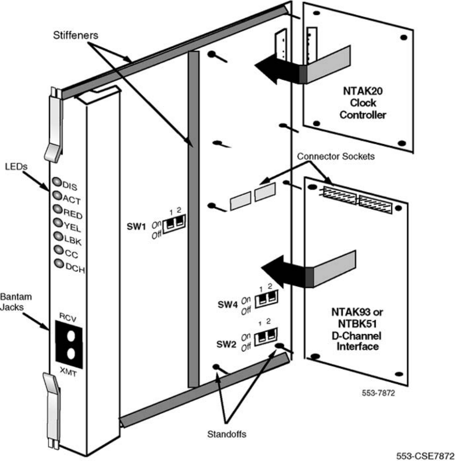
Figure 159: NTBK50 2.0 Mb PRI card with daughterboards
