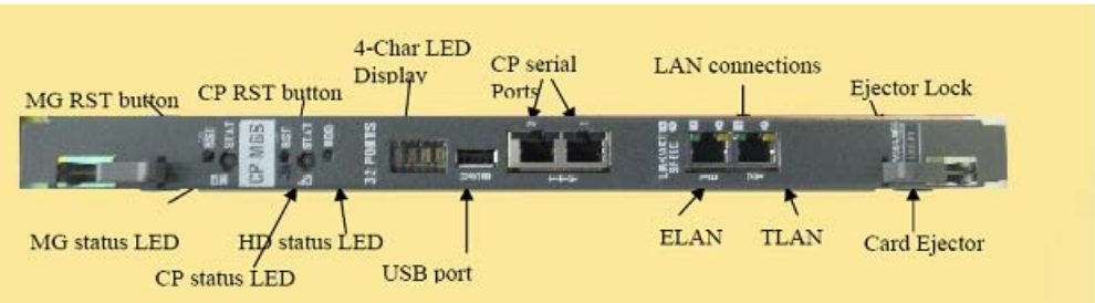
Figure 167: CP MG faceplate
