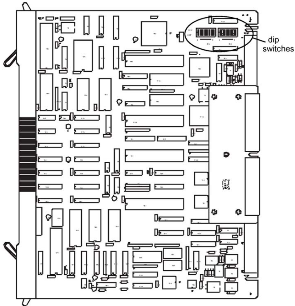
Figure 48: LEI card - E1 protocol dip switch locations
