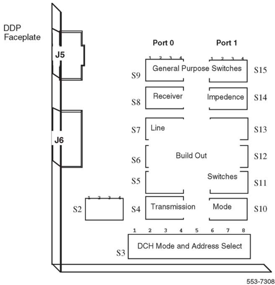
Figure 20: Switch functions and areas
