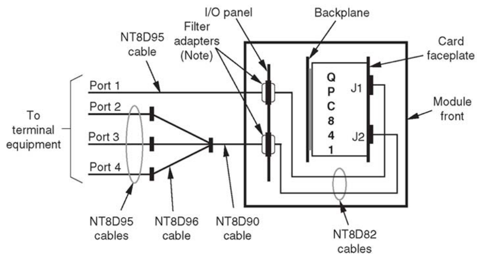
Figure 204: QPC841 QSDI card cabling
