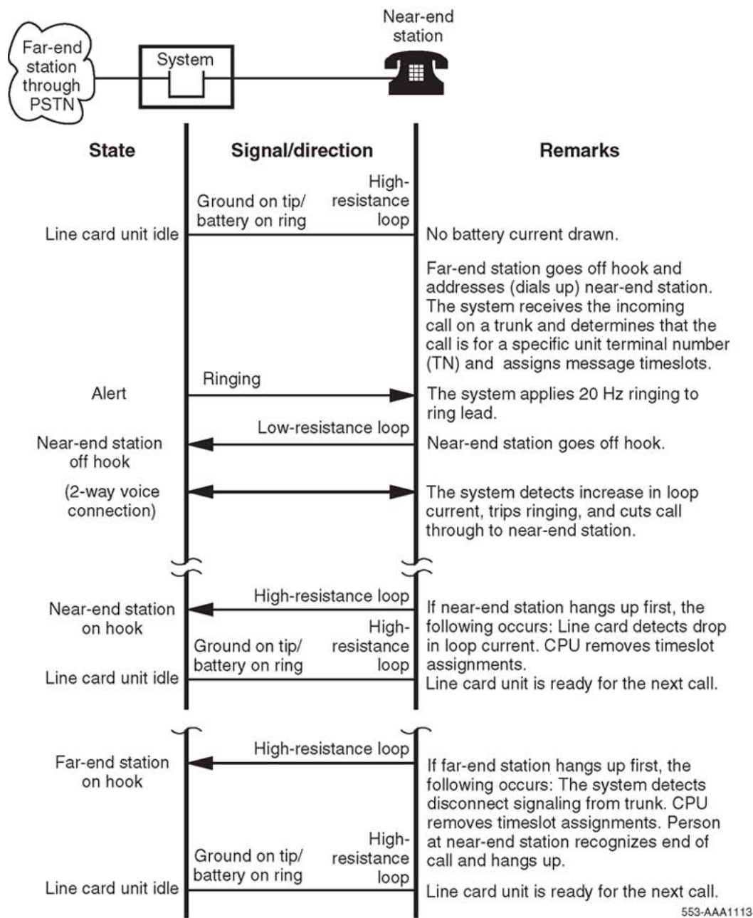
Figure 6: Call connection sequence - near-end station receiving call
