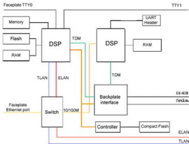
Figure 193: Voice Gateway Media card block diagram
