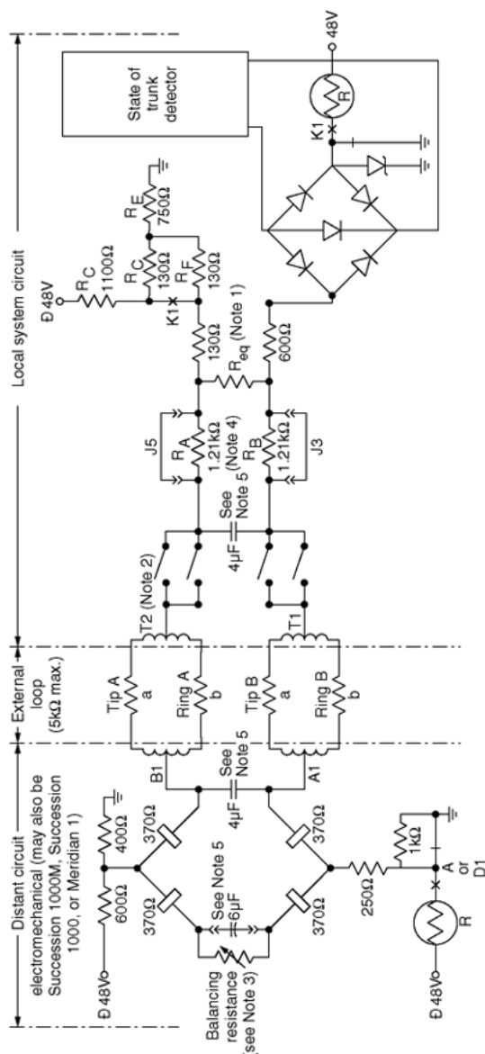
Figure 142: 4-wire DX signaling
