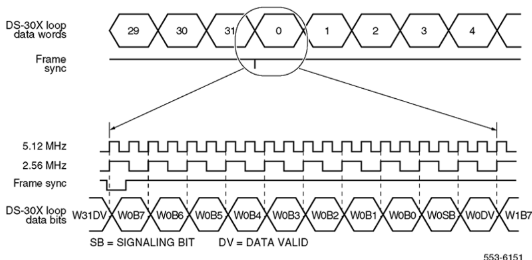
Figure 14: DS-30X loop data format
