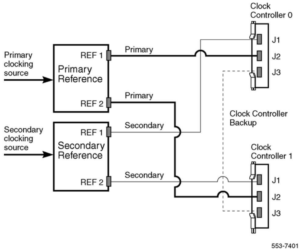
Figure 86: Clock Controller - Option 1
