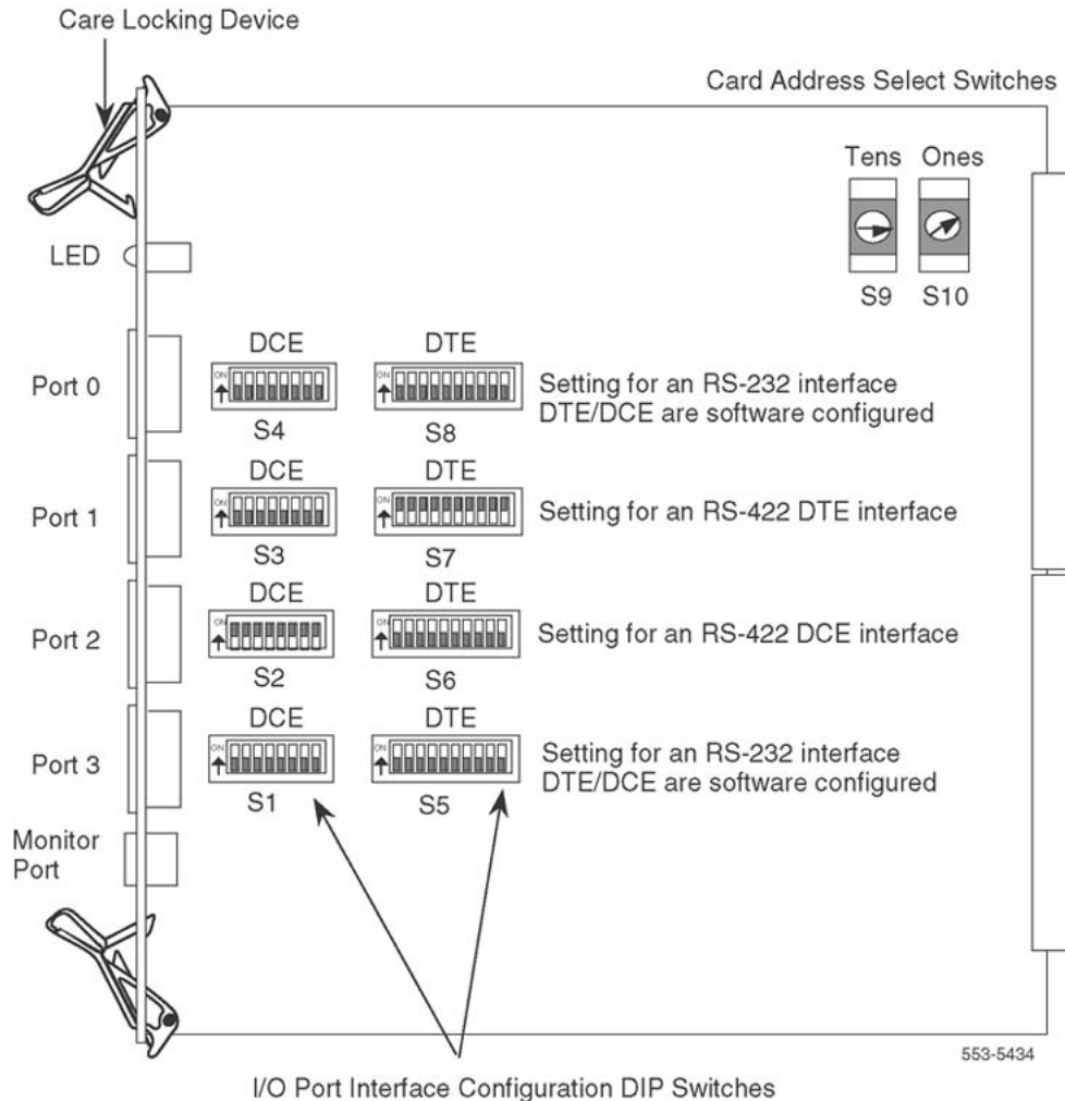
Figure 93: MSDL switch setting example
