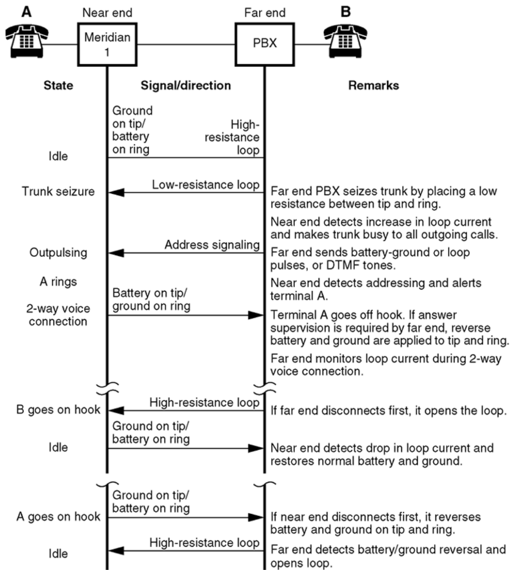
Figure 132: Two-way, loop OAID, TIE trunk call connection sequence - incoming call from far-end PBX
