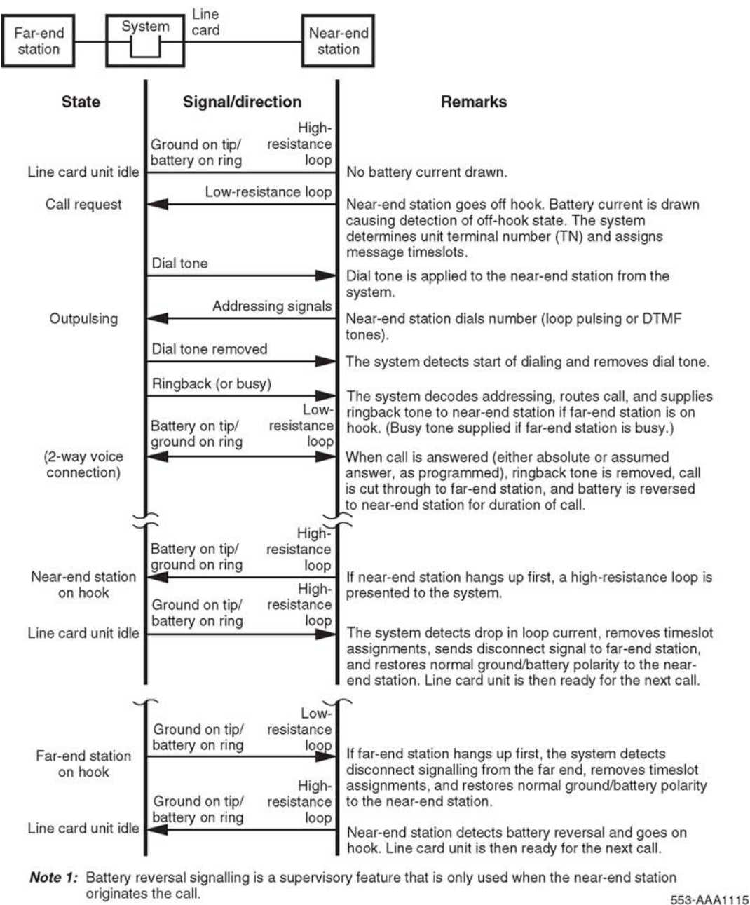
Figure 8: Battery reversal answer and disconnect supervision sequence
