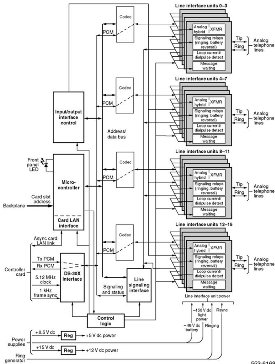
Figure 106: Analog message waiting line card - block diagram
