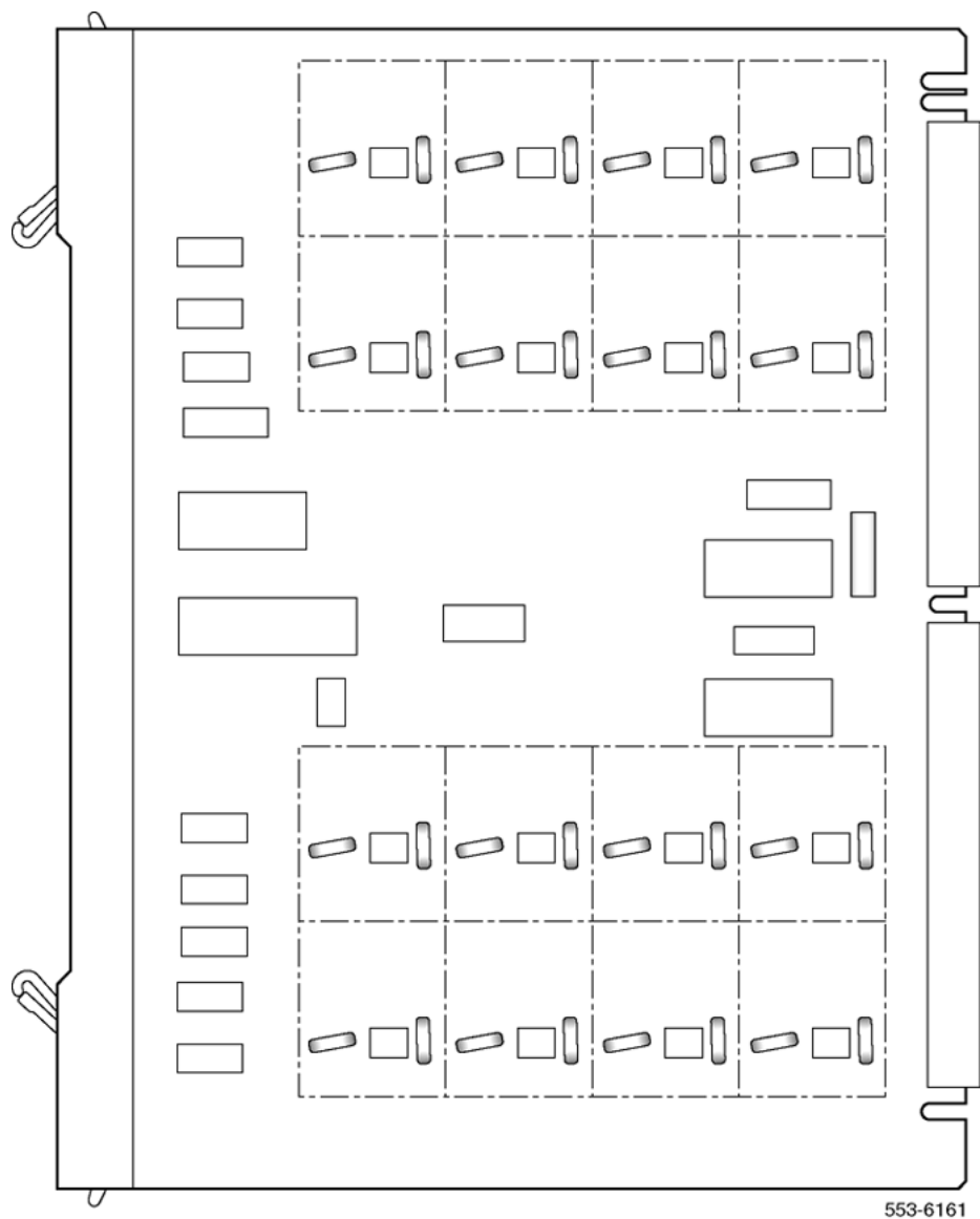
Figure 104: Digital line card - jumper block and switch locations
