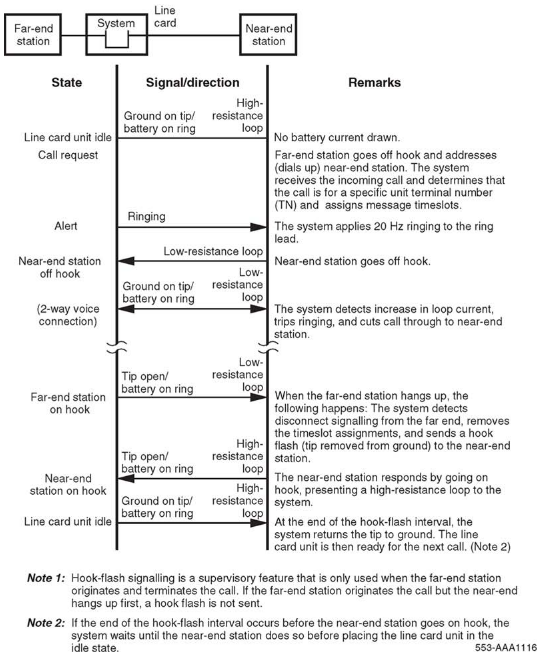
Figure 9: Hook flash disconnect supervision sequence
