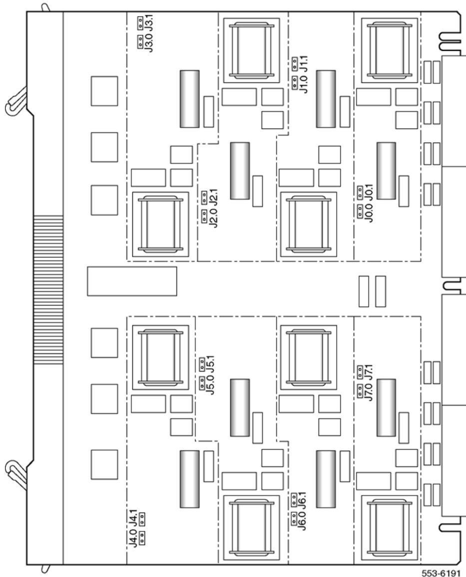
Figure 25: OPS analog line card - jumper block locations
