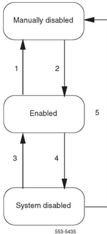
Figure 95: MSDL states
