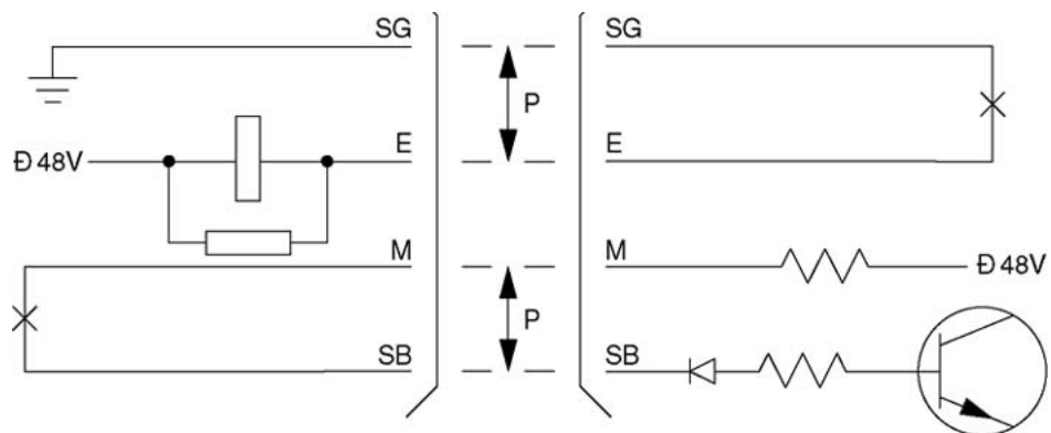
Figure 140: E and M Type I signaling
