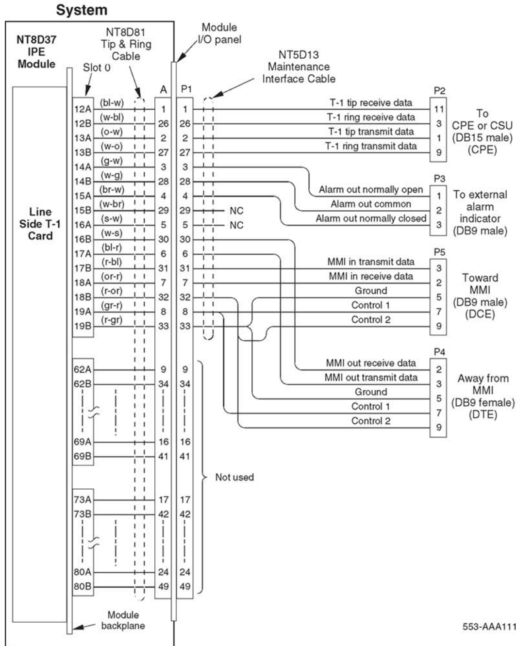
Figure 32: Lineside T1 card - connection using the NTSD13AA Lineside T1 cable
