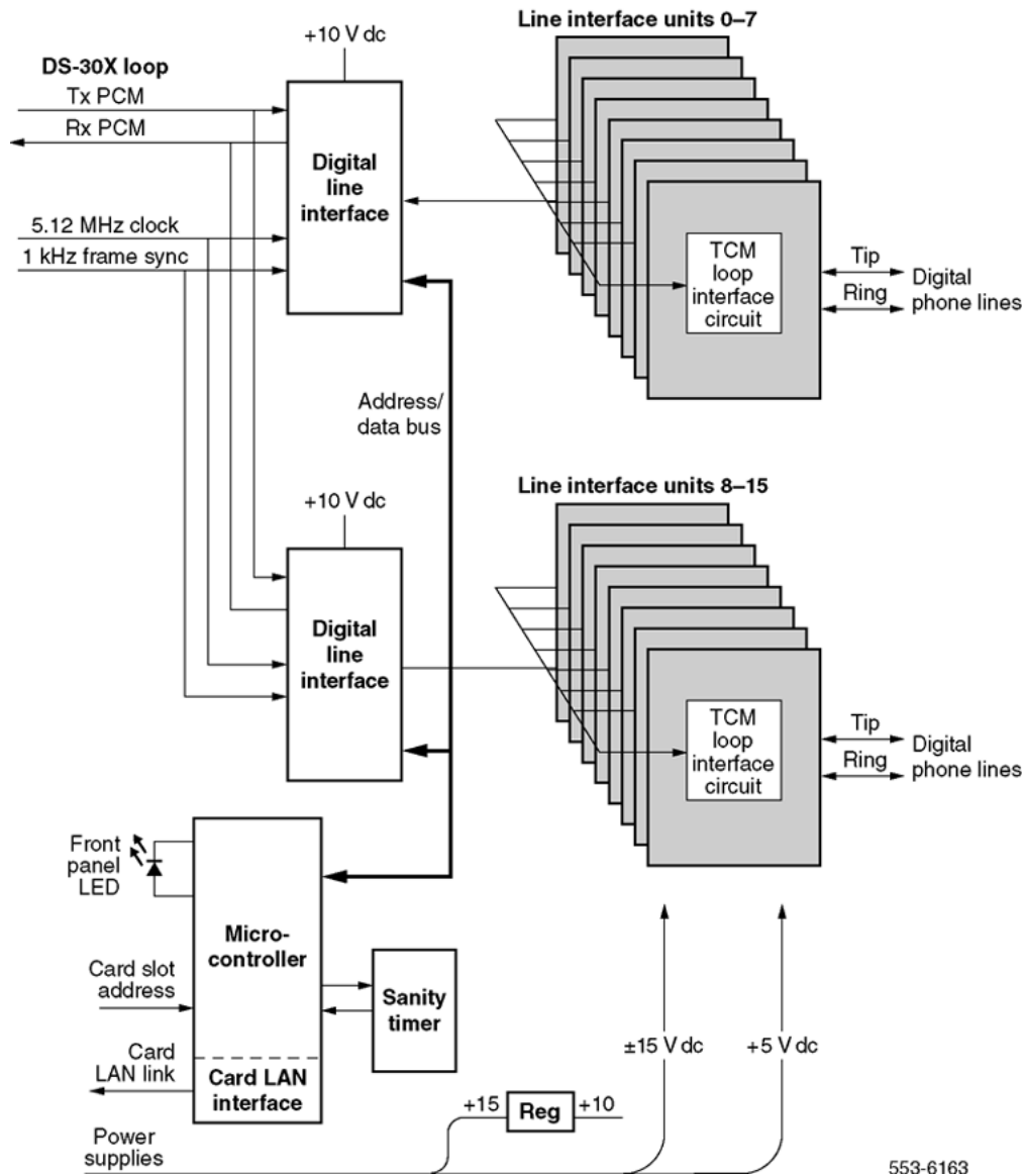
Figure 101: Digital line card - block diagram
