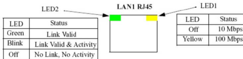
Figure 189: ELAN and TLAN port LED indicators
