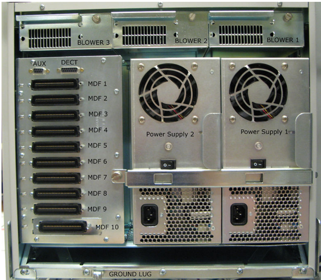
Figure 200: MG 1010 rear view
