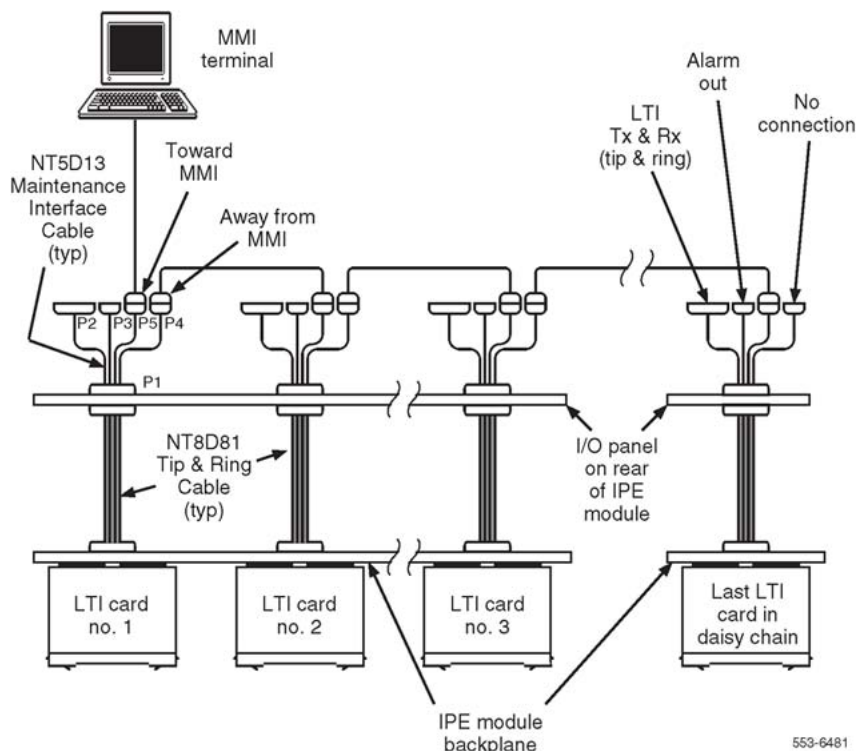
Figure 33: Lineside T1 card - connecting two or more cards to the MMI
