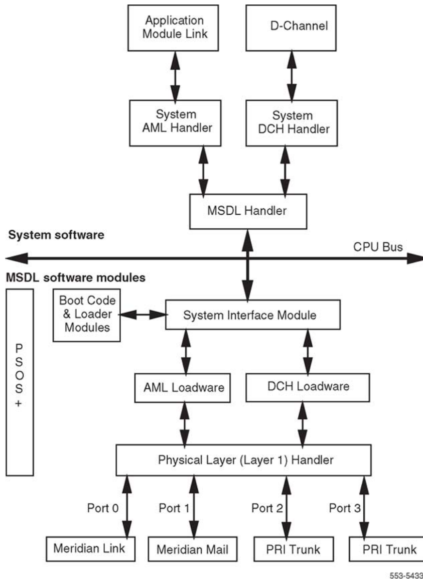
Figure 92: MSDL functional block diagram
