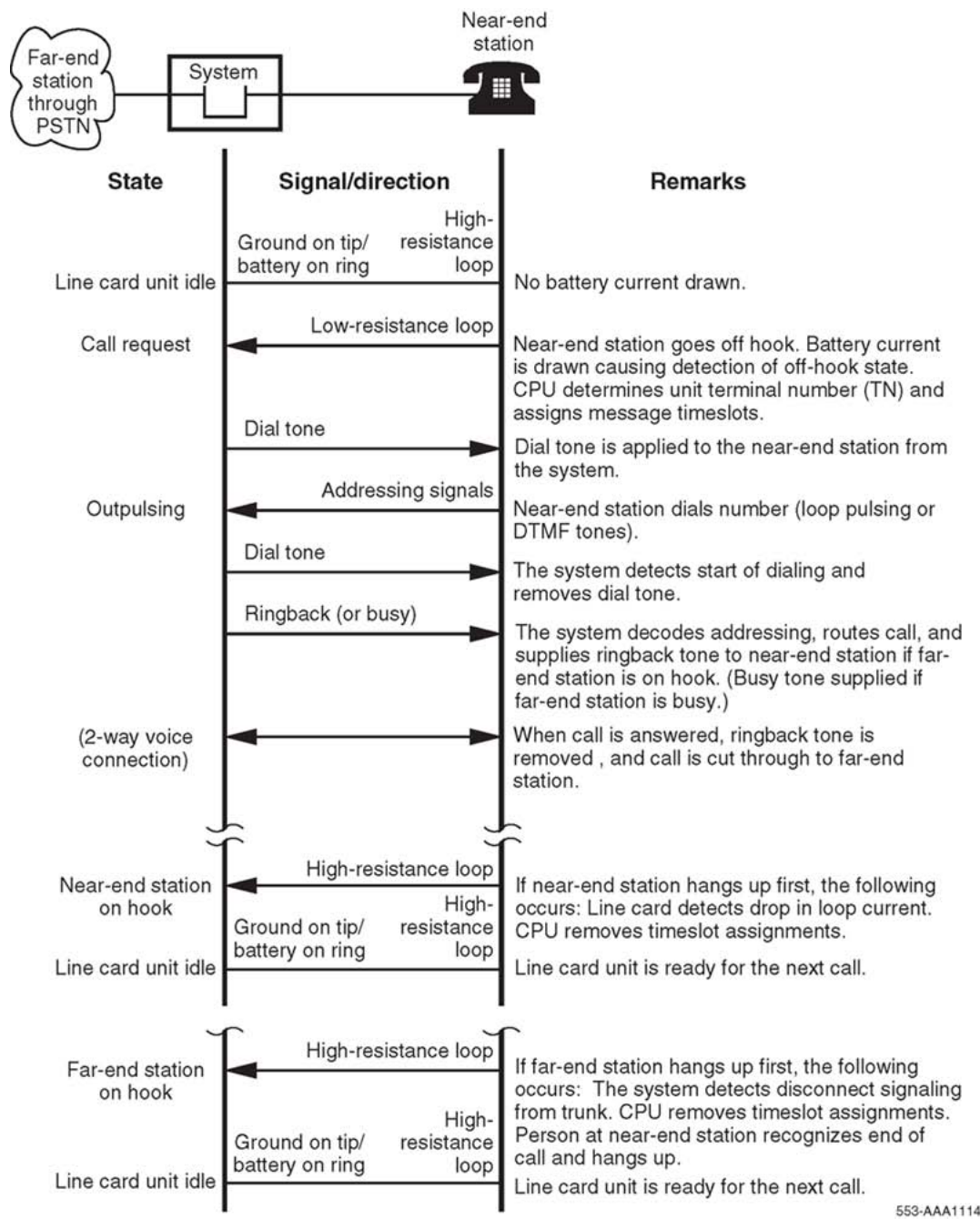
Figure 7: Call connection sequence - near-end originating call
