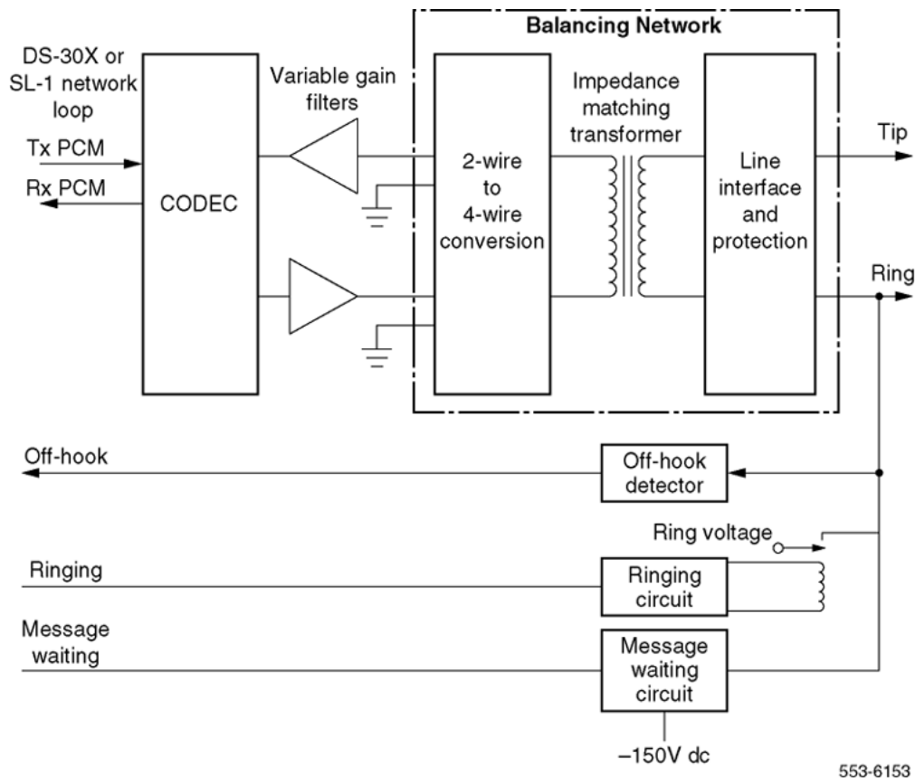
Figure 4: Typical analog line interface unit block diagram
