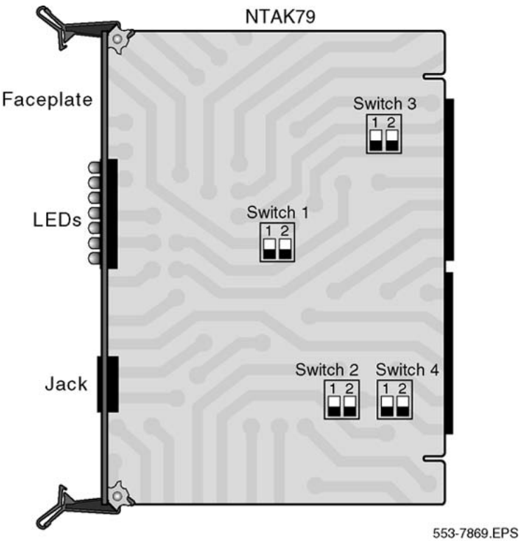
Figure 153: NTA79 card with switch locations
