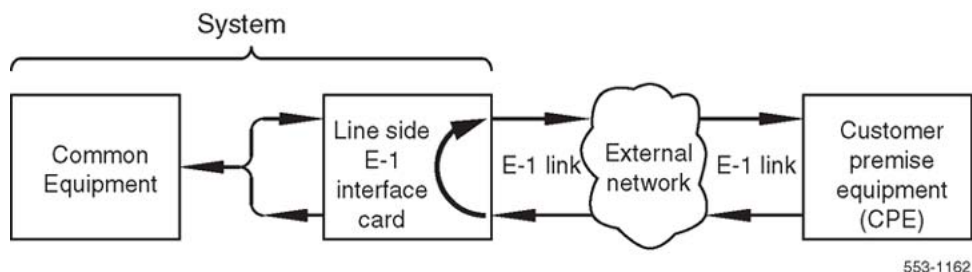
Figure 40: MMI network loopback test
