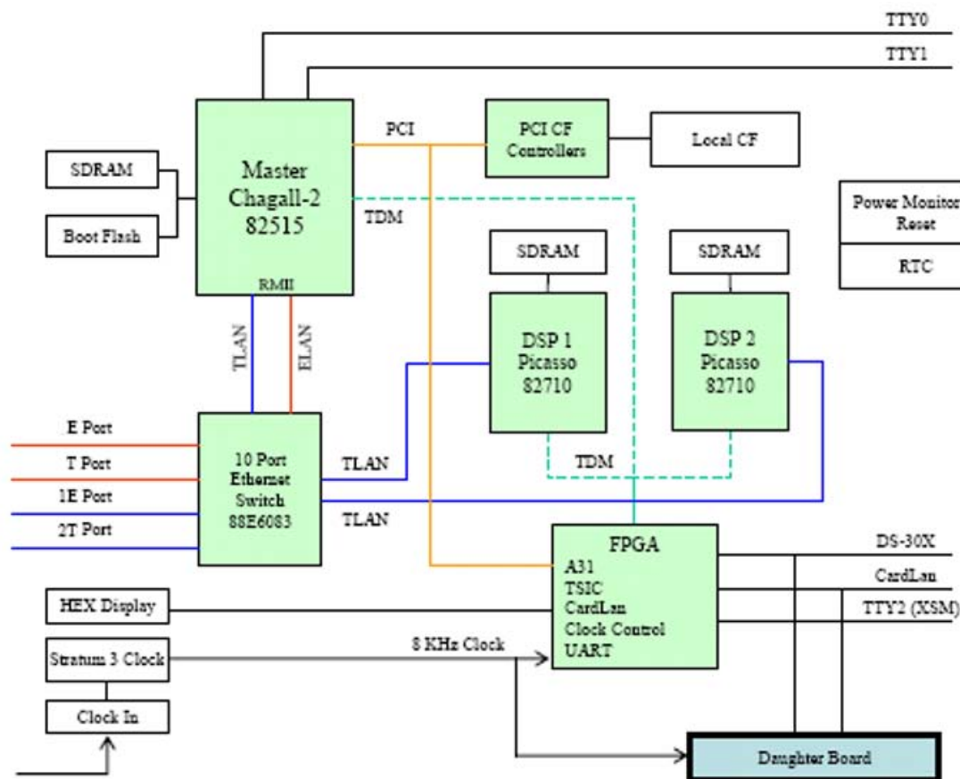
Figure 164: MG XPEC block diagram
