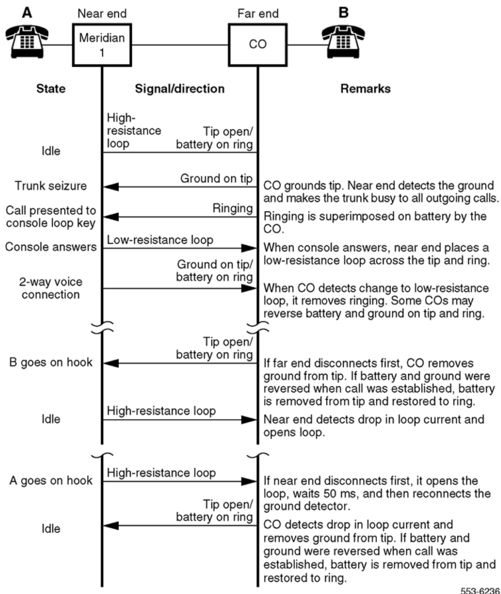
Figure 114: Ground start call connection sequence - incoming call from CO/FX/WATS
