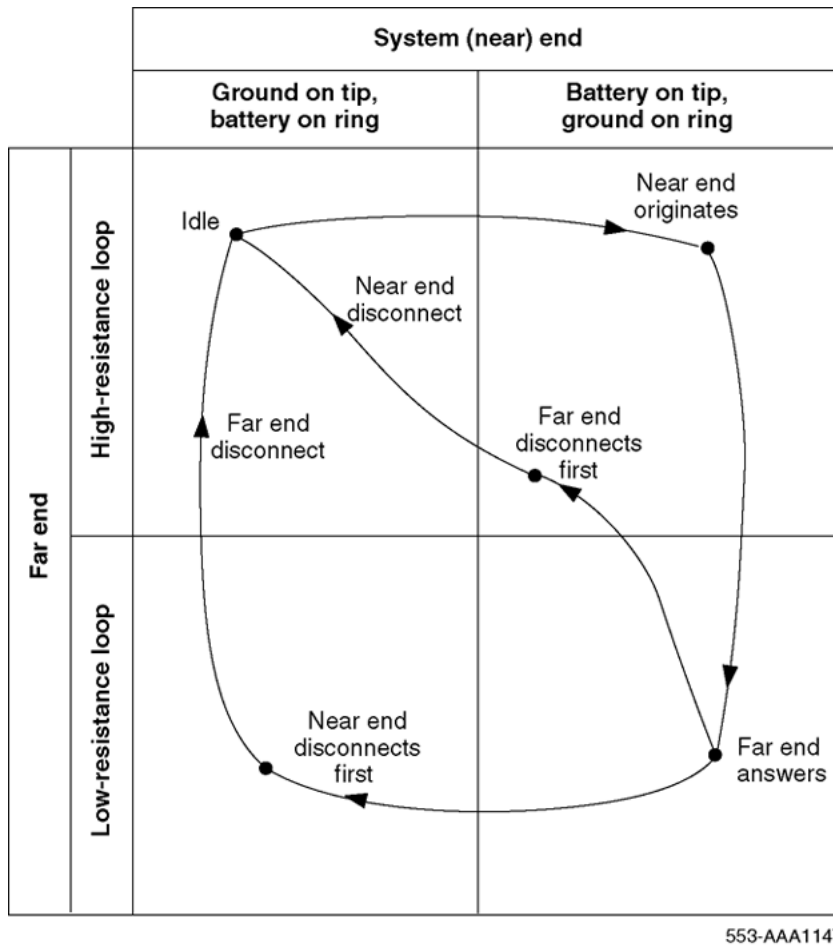
Figure 131: Two-way, loop OAID, TIE trunk call states - outgoing call to far-end PBX
