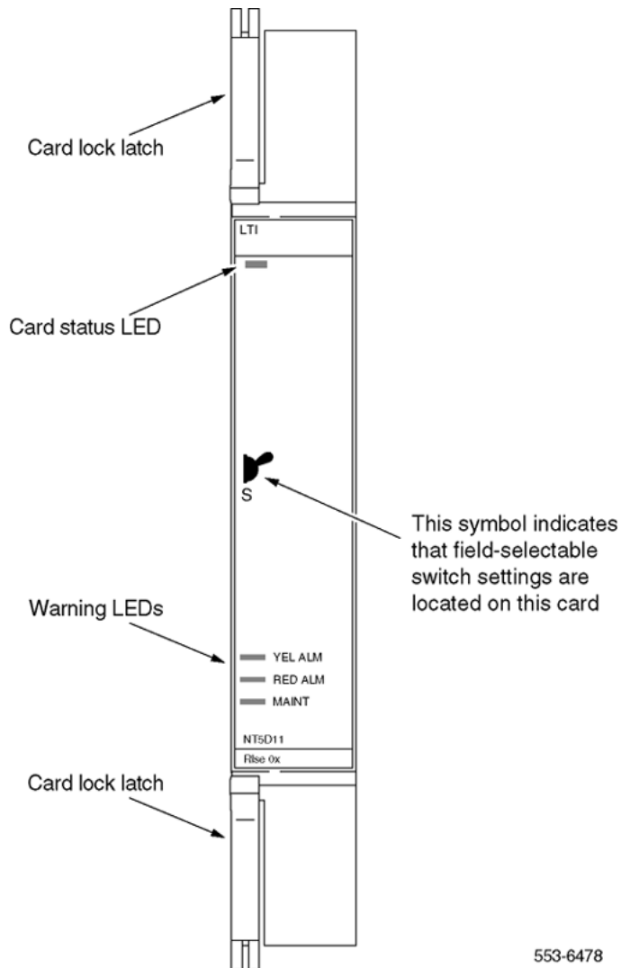
Figure 29: Lineside T1 card faceplate
