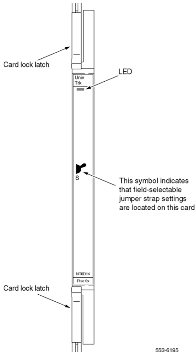
Figure 109: Universal trunk card - faceplate
