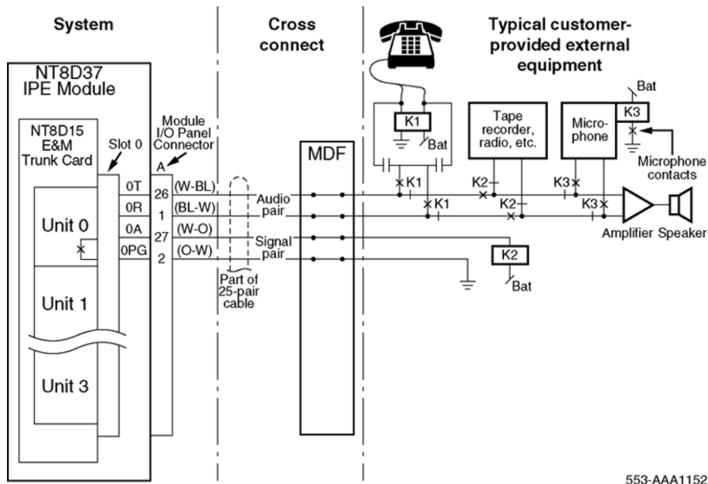
Figure 143: Paging trunk operation
