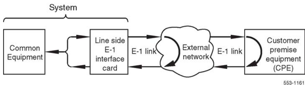
Figure 68: MMI External loopback test
