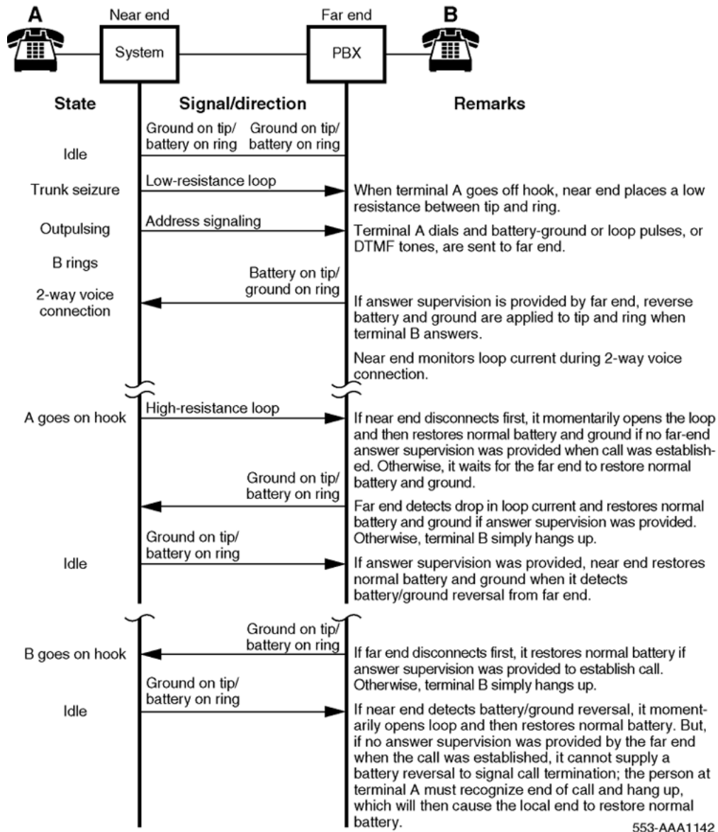
Figure 124: Two-way, loop DR, TIE trunk call connection sequence - outgoing call to far-end PBX
