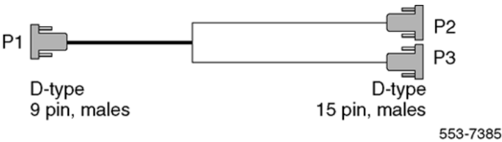
Figure 74: NTCK45AA
