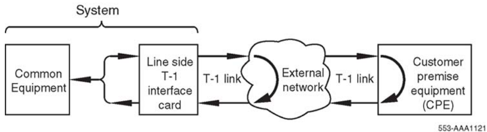
Figure 39: MMI external loopback test
