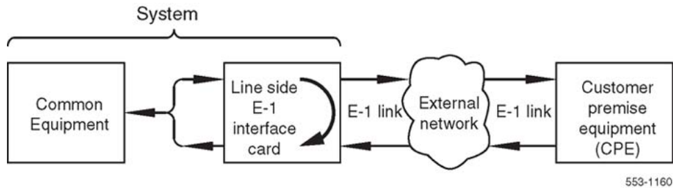
Figure 67: MMI Local loopback test
