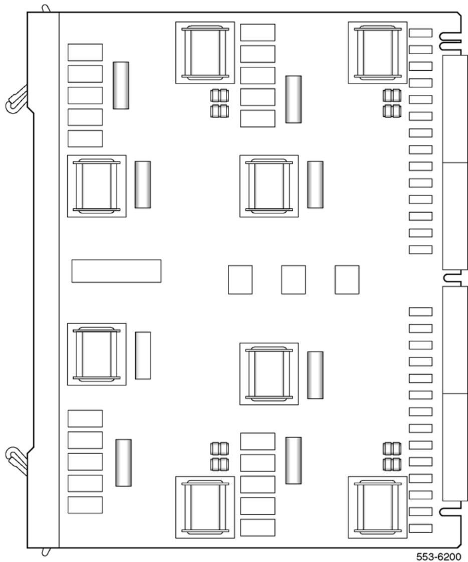
Figure 150: E and M Trunk card - jumper locations
