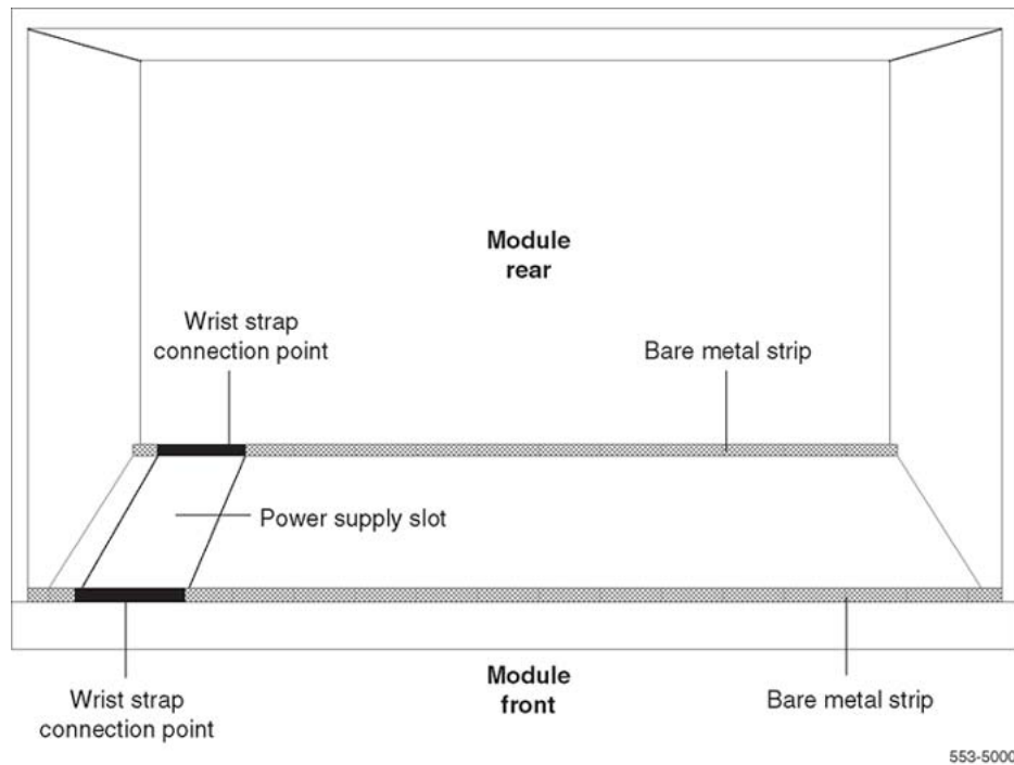
Figure 17: Static discharge points
