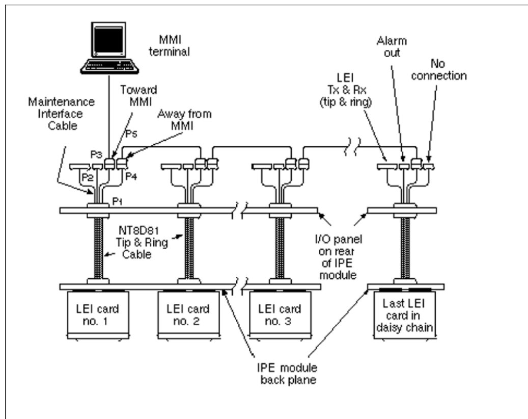
Figure 49: LEI card - connecting two or more cards to the MMI
