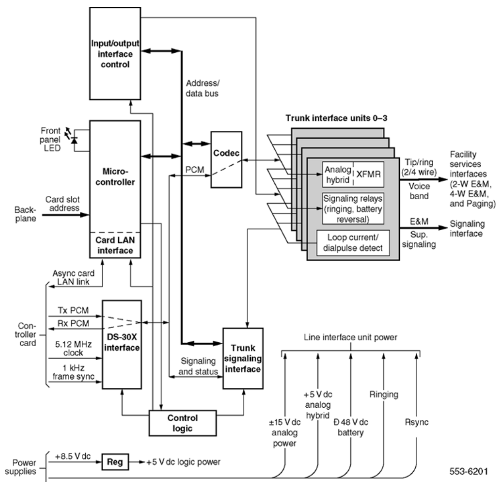
Figure 139: E and M Trunk card - block diagram
