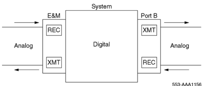
Figure 151: Pad orientation
