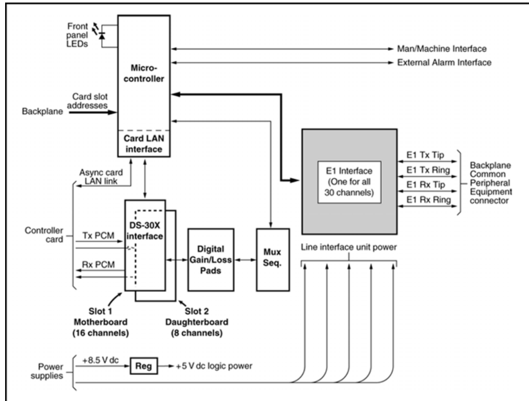
Figure 46: LEI card - block diagram
