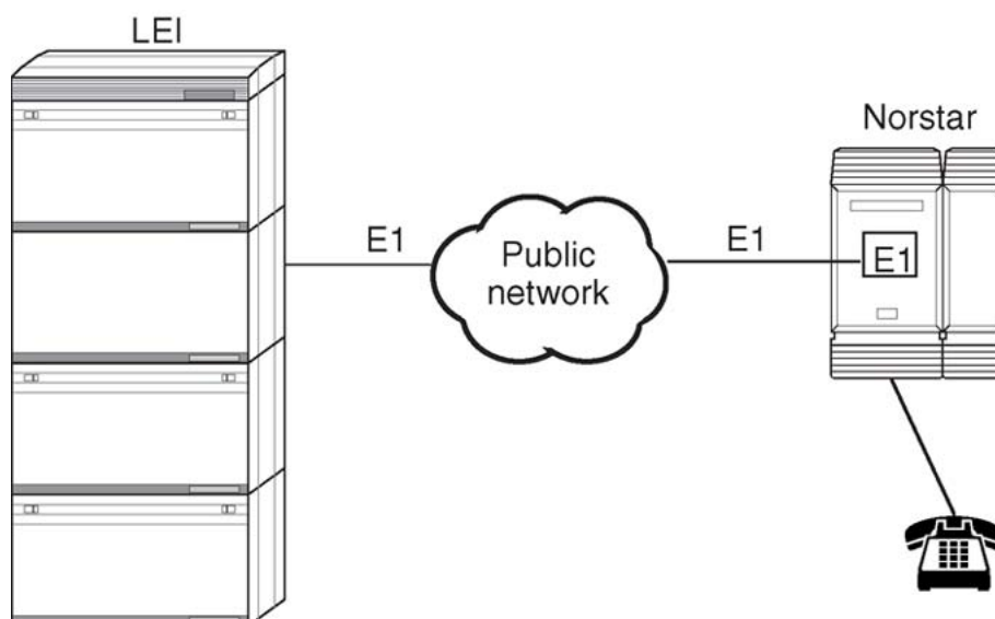
Figure 72: LEI connection to Norstar system
