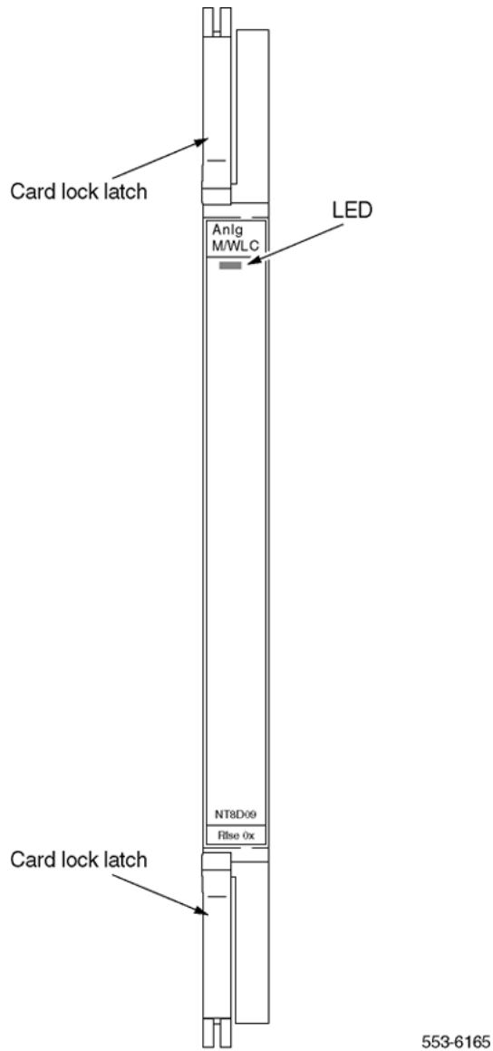
Figure 105: Analog message waiting line card - faceplate
