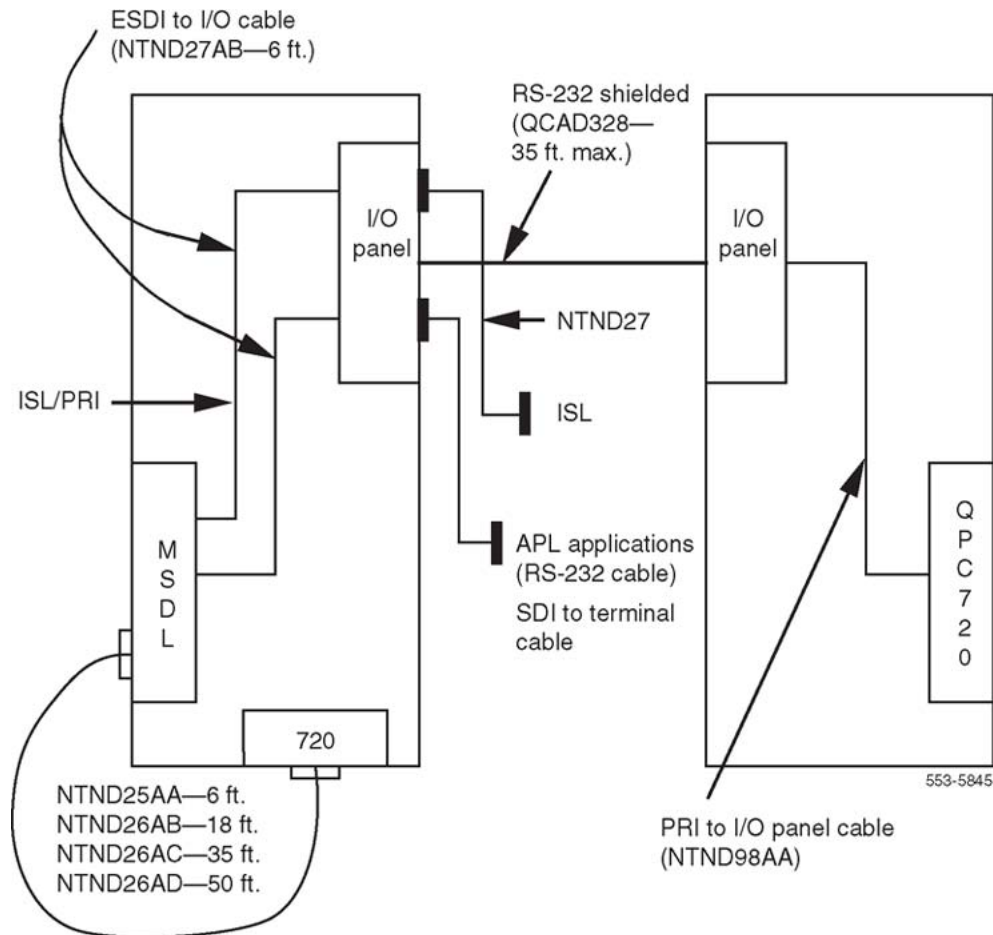
Figure 94: MSDL cabling
