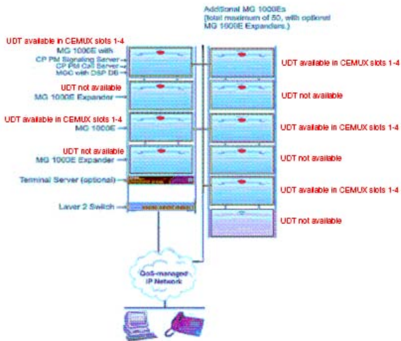
Figure 156: UDT card positioning in a CS 1000E system
