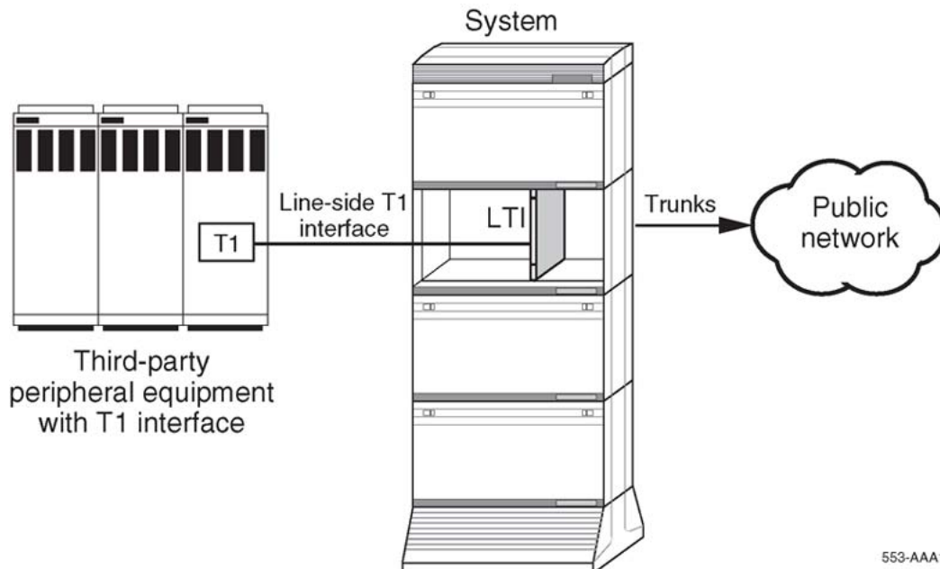
Figure 41: Lineside T1 interface connection to IPE
