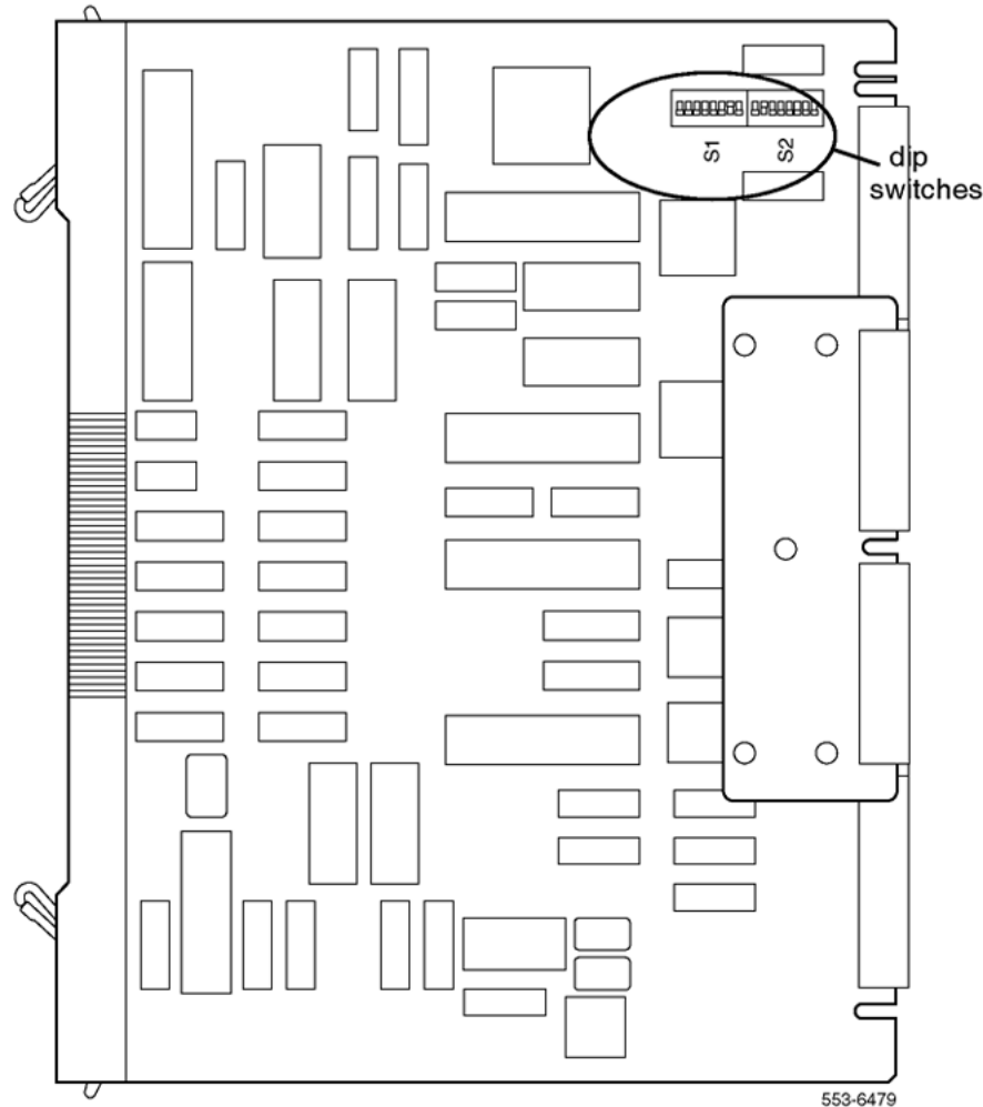
Figure 31: Lineside T1 card - T1 protocol dip switch locations
