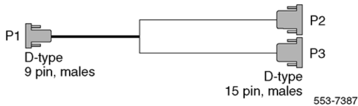
Figure 79: NTCK46AA/AB/AC/AD
