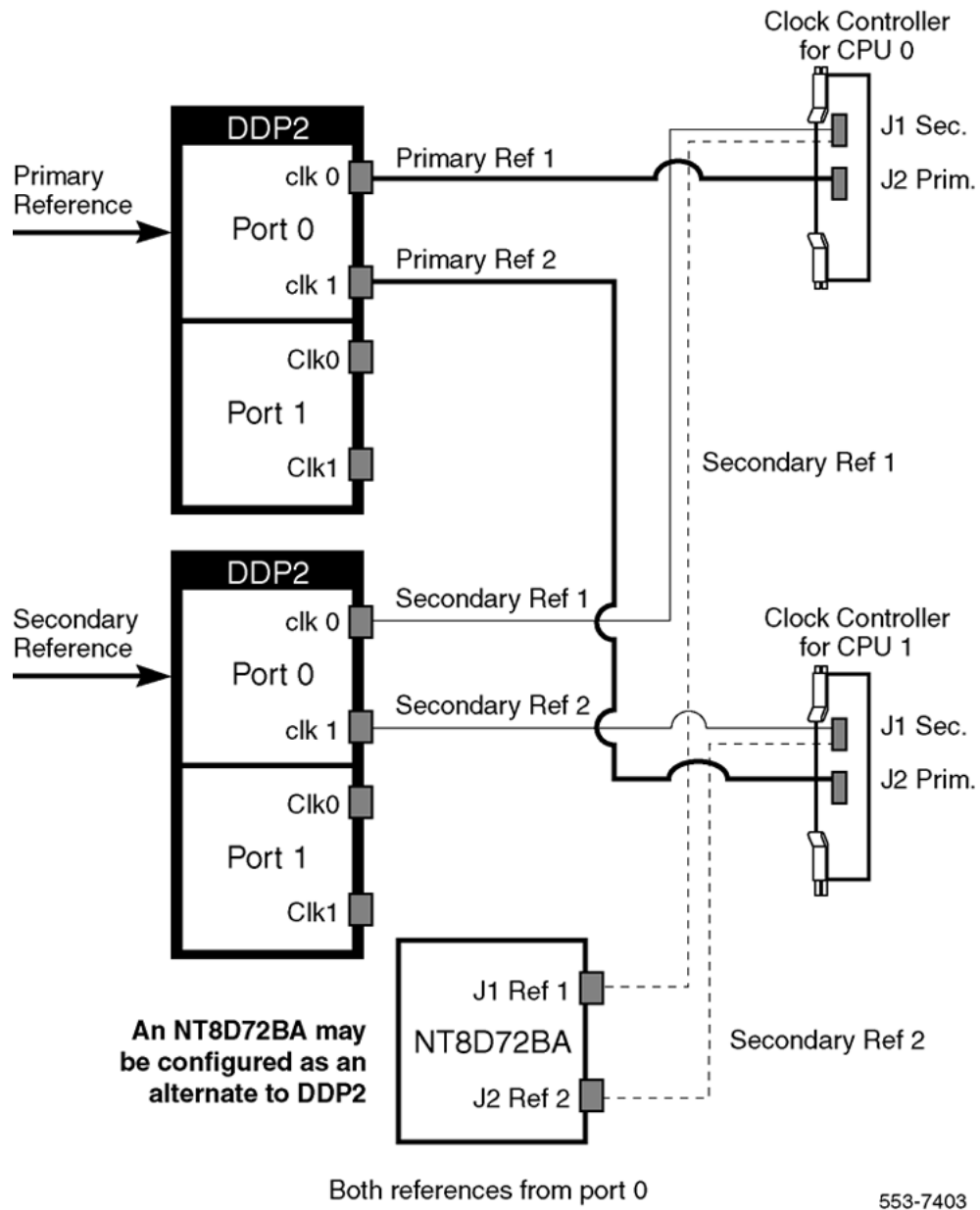
Figure 87: Clock Controller - Option 2
