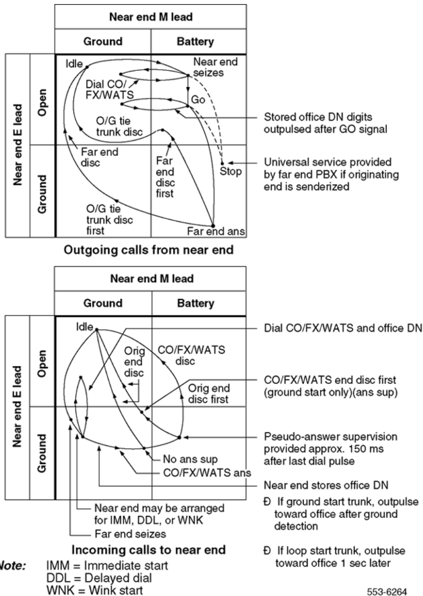
Figure 146: E and M Type I signaling patterns - originating party release on a tandem connection
