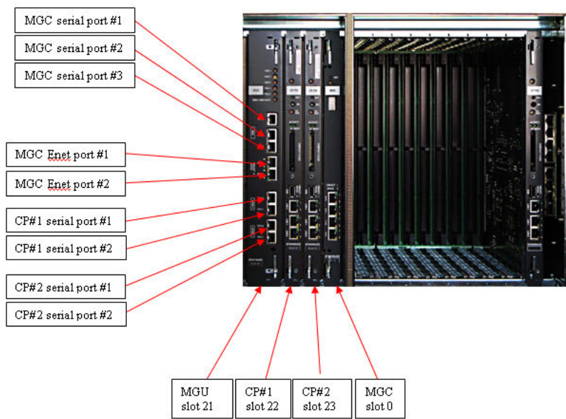
Figure 198: NTC314AAE6 utility card
