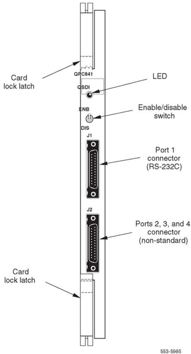
Figure 201: QPC841 QSDI card front panel
