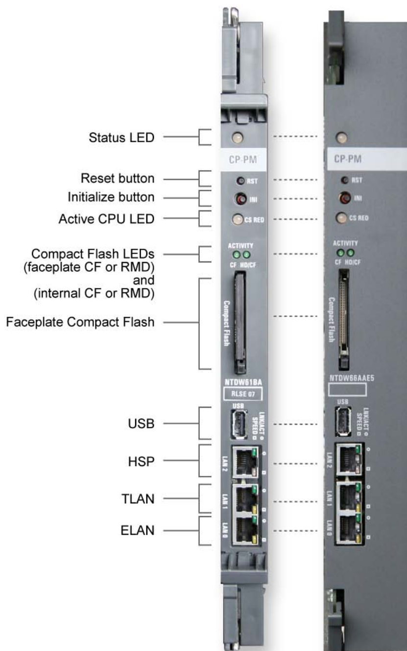
Figure 188: CP PM NTDW61 and NTDW66 faceplates
