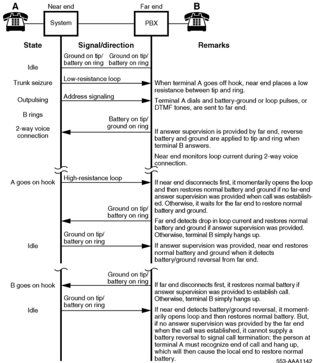
Figure 126: Two-way, loop DR, TIE trunk call connection sequence - outgoing call to far-end PBX
