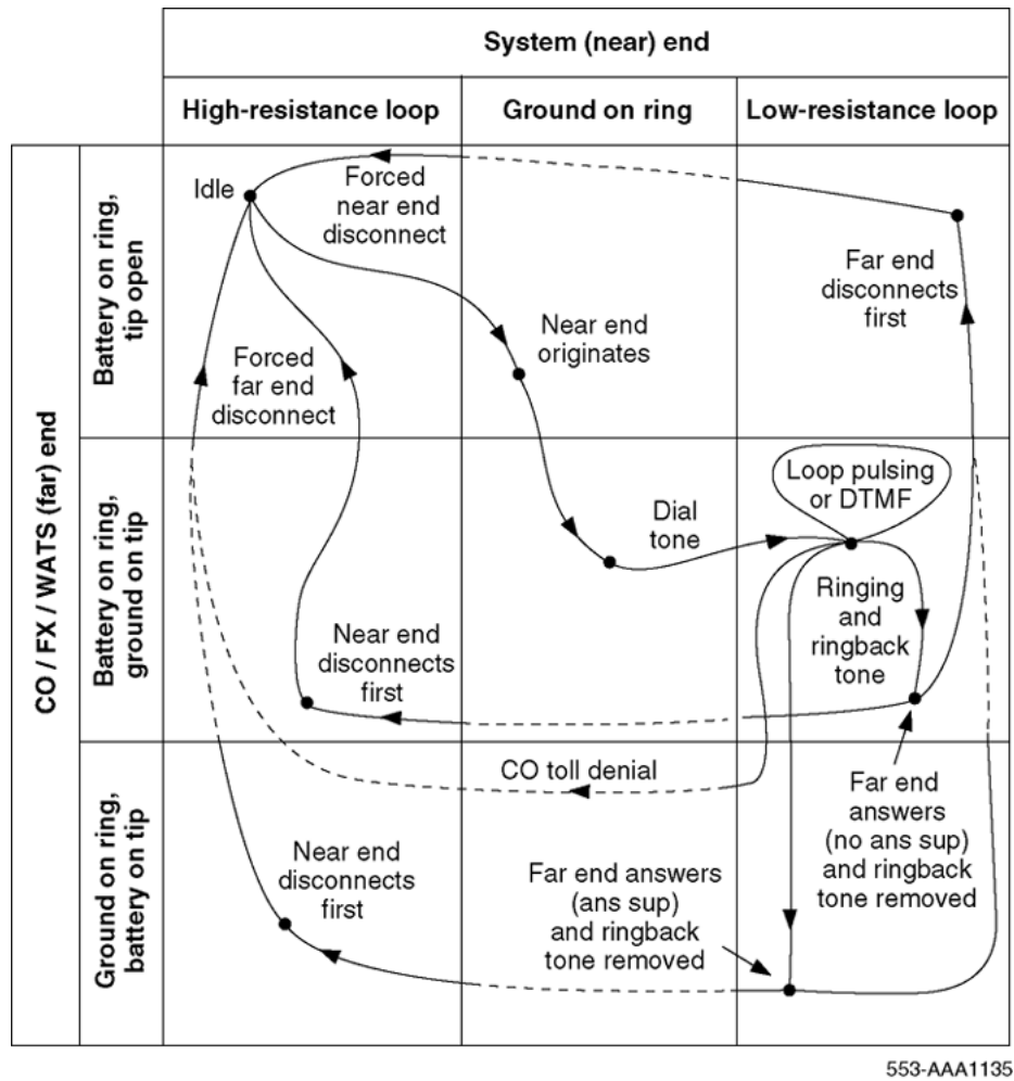
Figure 117: Ground start call states - outgoing call to CO/FX/WATS
