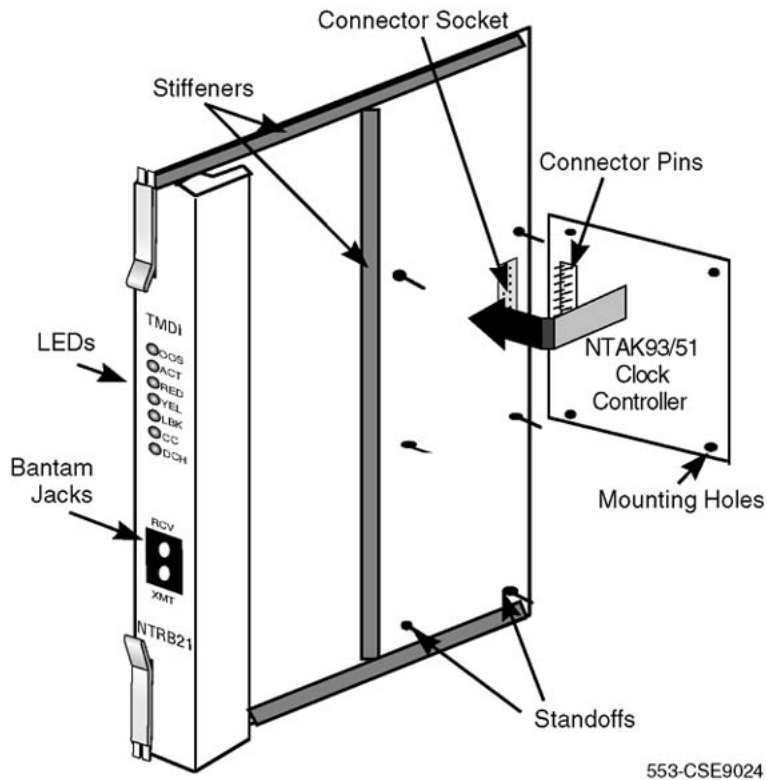
Figure 194: NTRB21 TMDI card with clock controller
