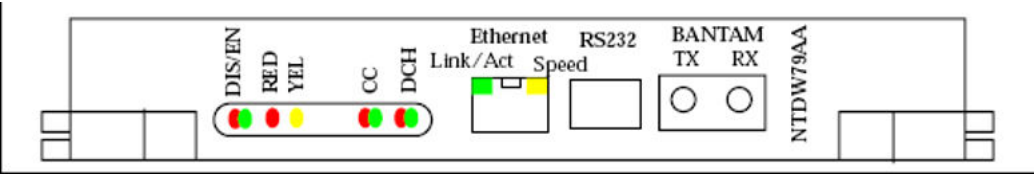
Figure 158: UDT card faceplate LEDs
