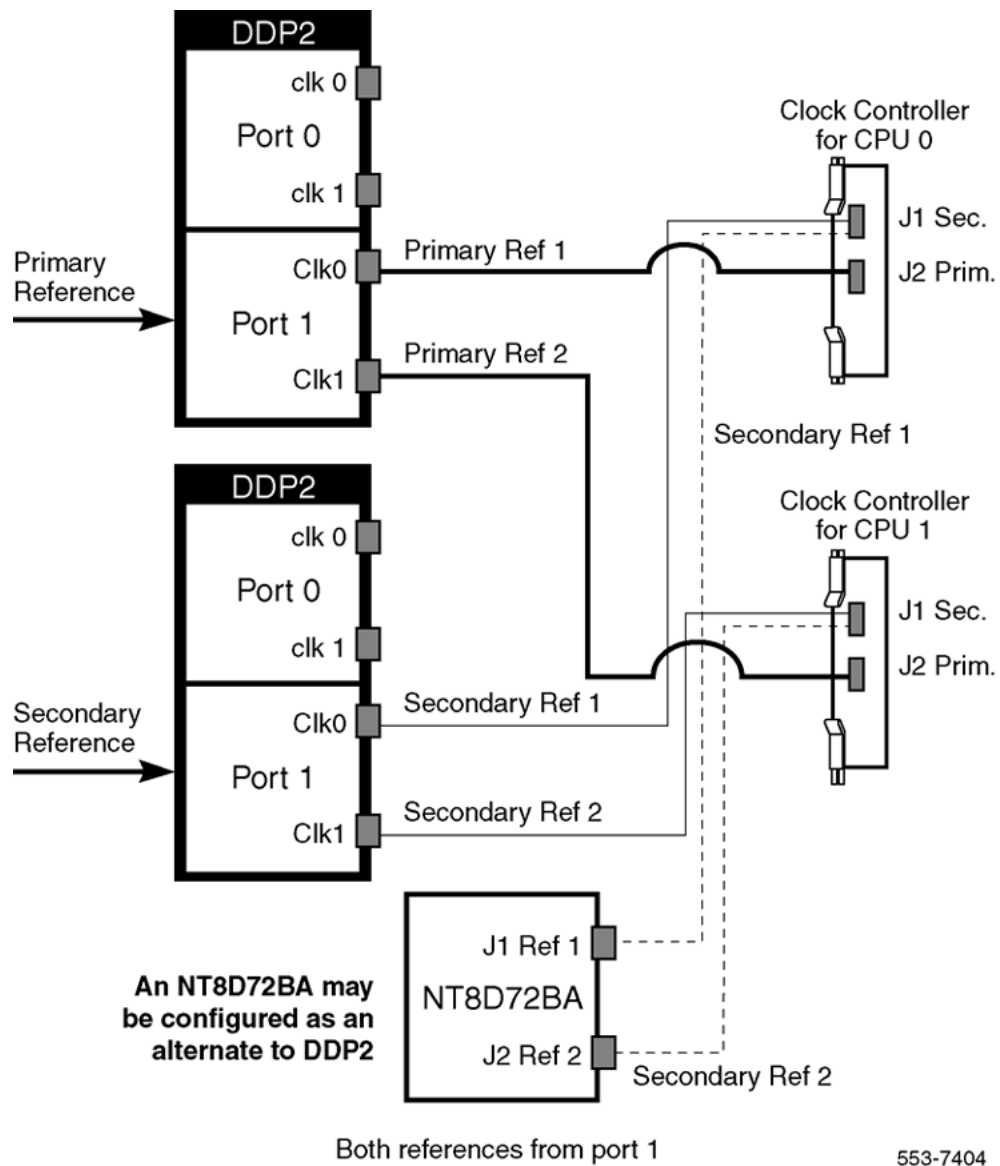
Figure 88: Clock Controller - Option 3
