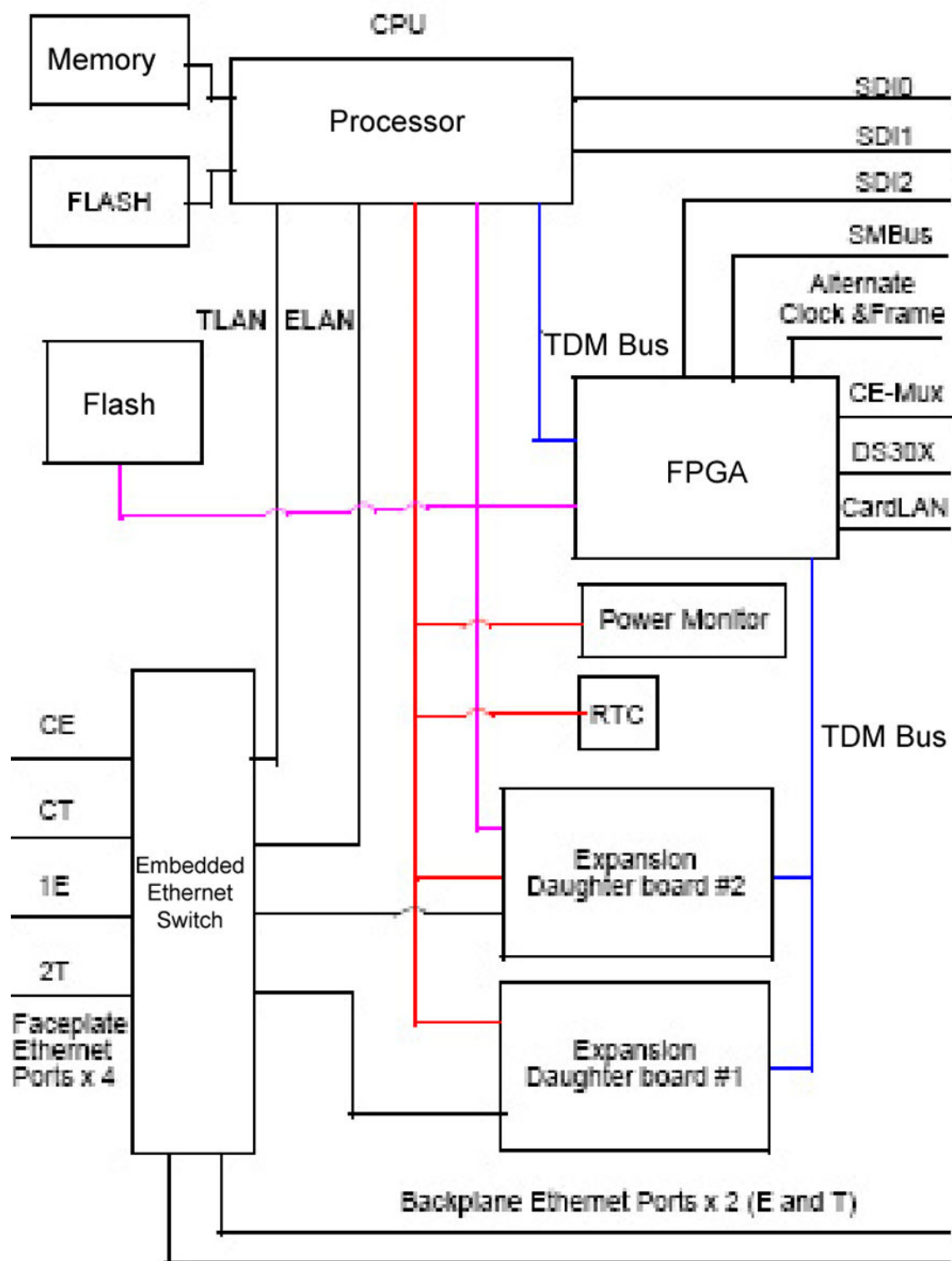
Figure 163: MGC block diagram
