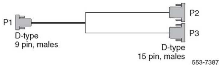
Figure 80: NTCK80AA/AB/AC/AD
