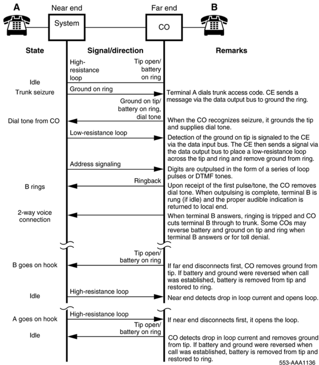
Figure 118: Ground start call connection sequence - outgoing call to CO/FX/WATS
