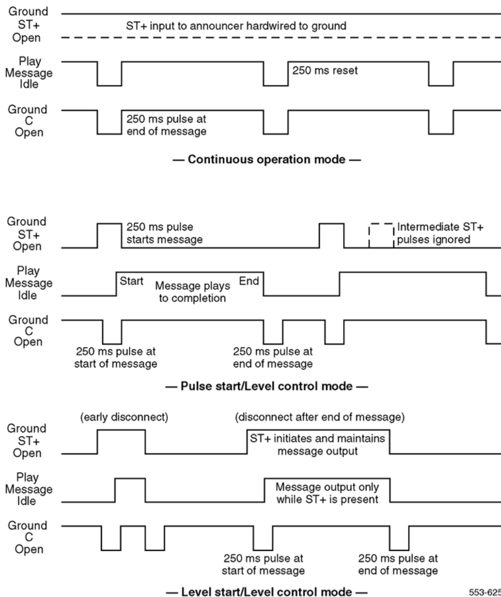
Figure 134: RAN control signals (Control GRD = IDLE)
