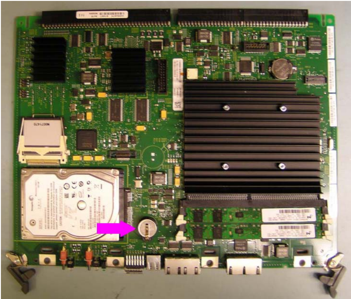
Figure 170: CP MG Security Device (Dongle)
