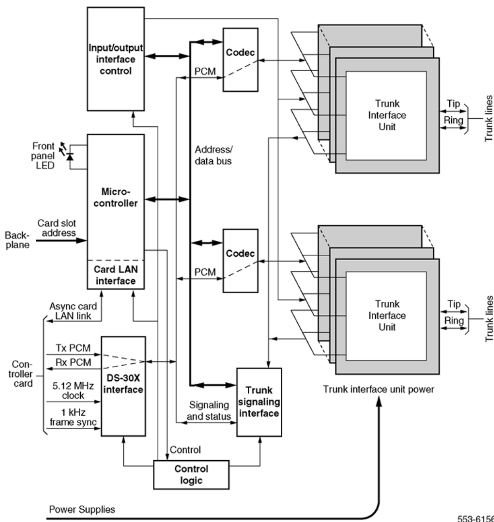
Figure 13: Typical IPE trunk card architecture
