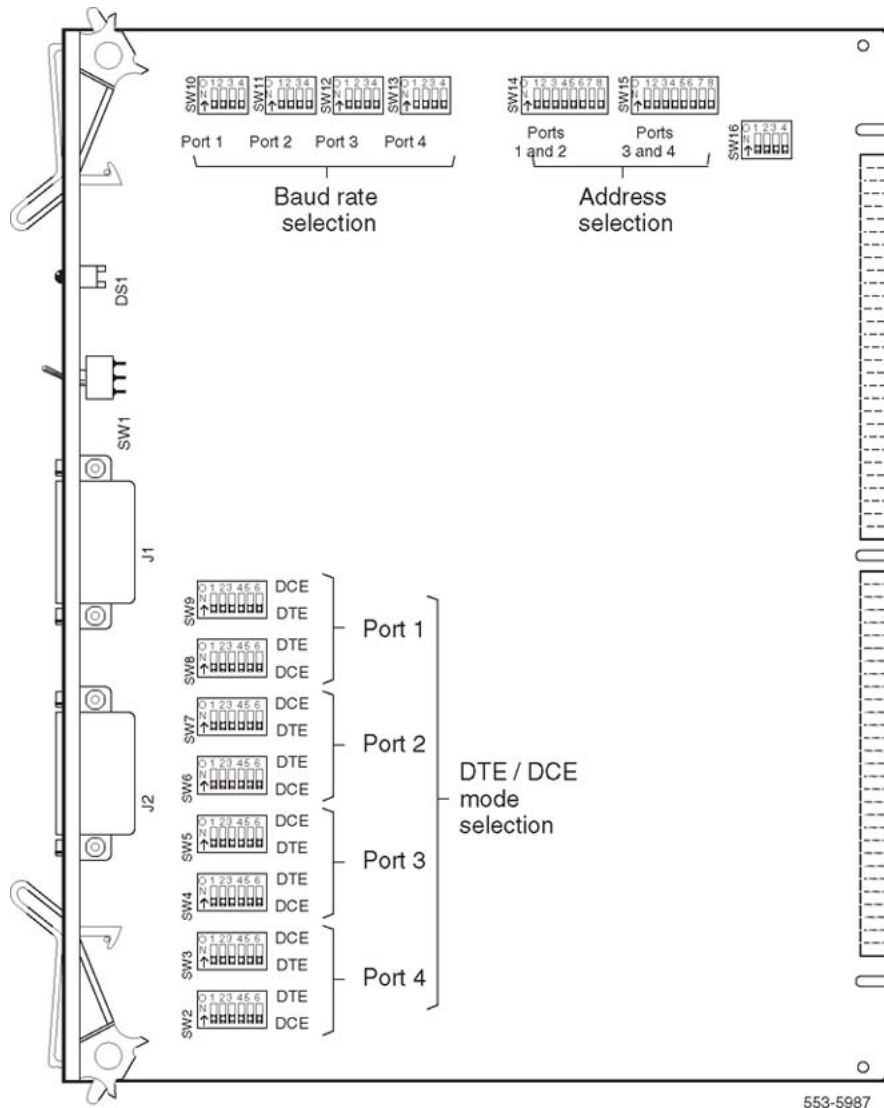
Figure 203: QSDI card option switch locations
