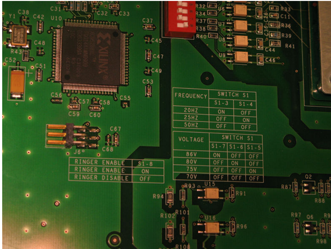
Figure 199: MGU dip switch settings
