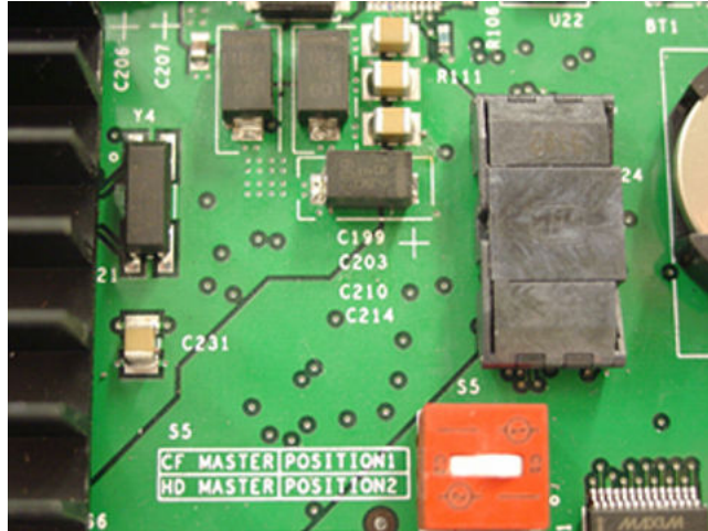
Figure 180: CP PM Signaling Server FMD dip switch
