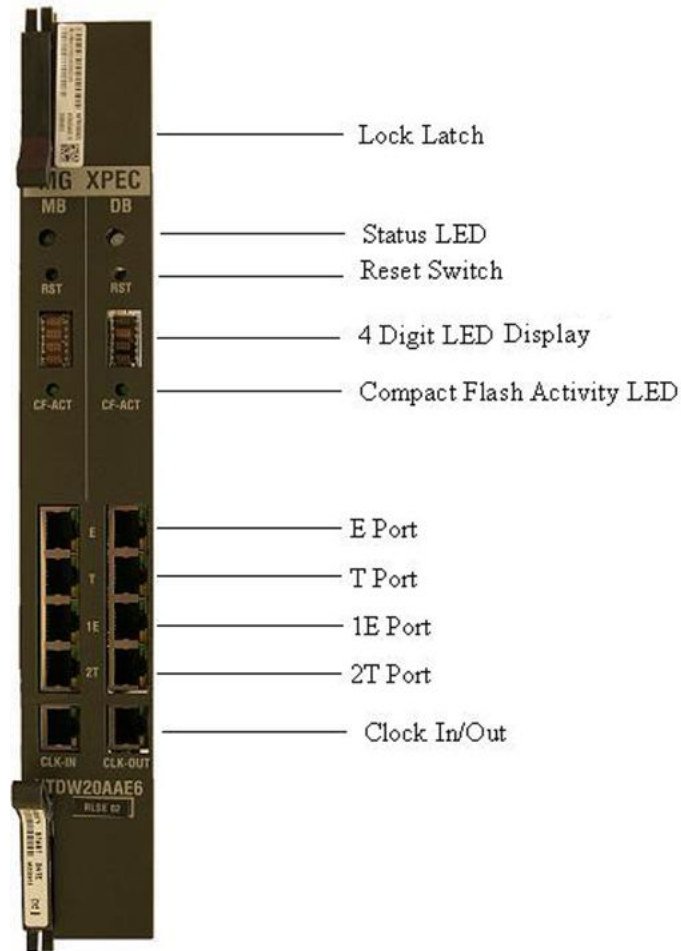
Figure 165: MG XPEC faceplate
