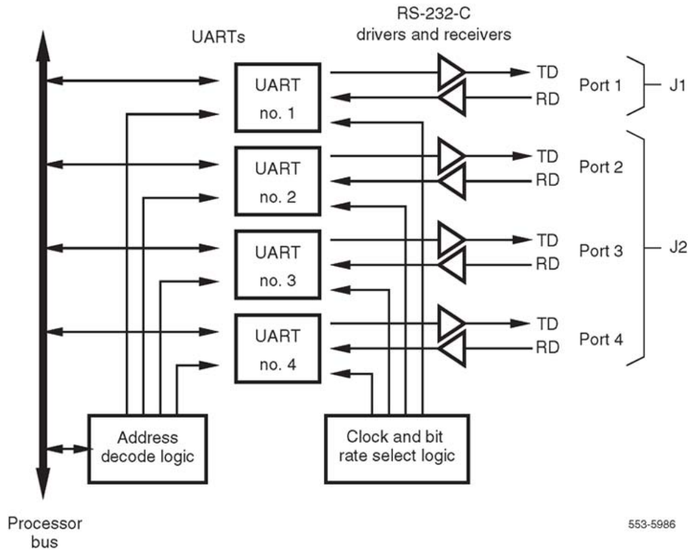
Figure 202: QPC841 QSDI card block diagram
