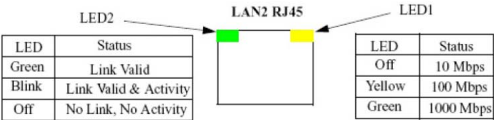
Figure 172: CP MG Ethernet port LED indicators
