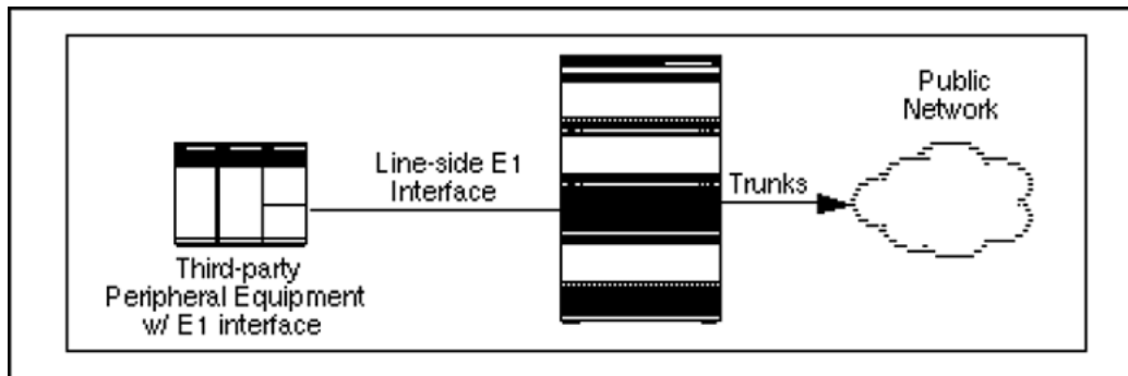
Figure 70: LEI connection to IPE
