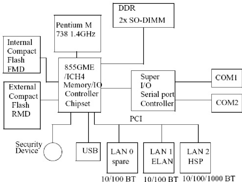
Figure 175: CP PM high level hardware block diagram
