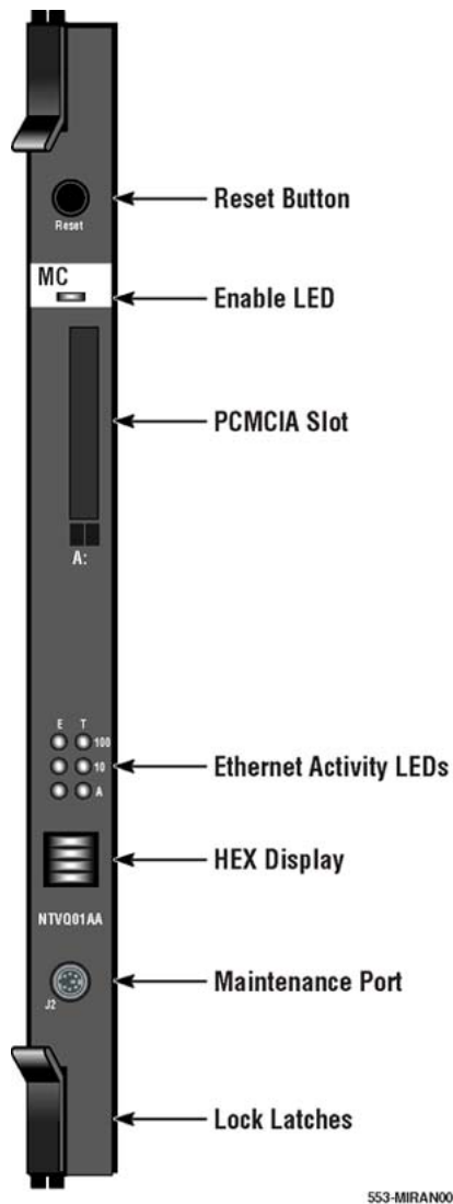
Figure 197: NTVQ01xx Media Card faceplate
