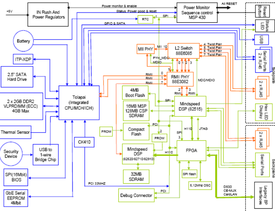
Figure 166: CP MG hardware block diagram
