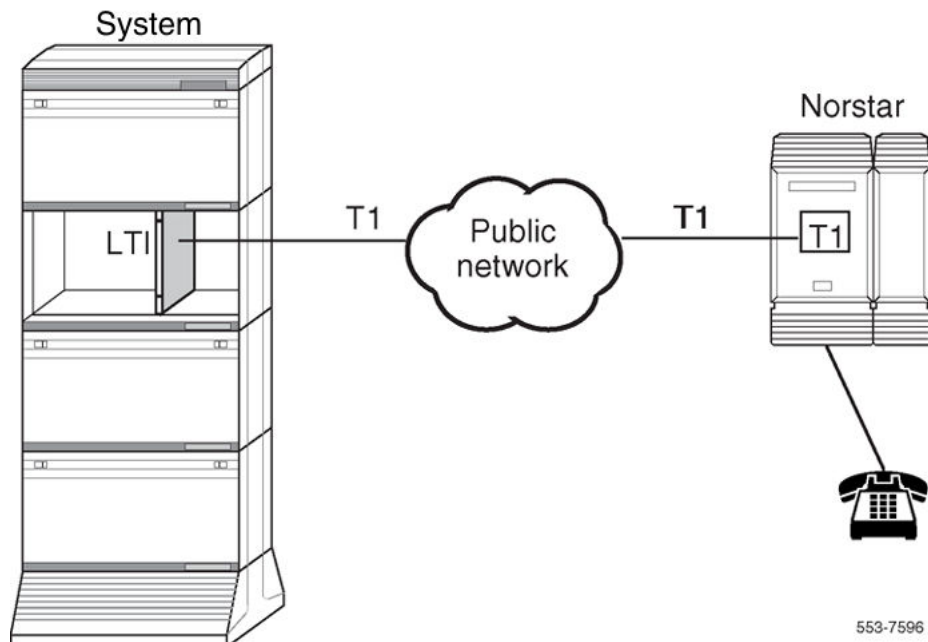
Figure 43: Lineside T1 interface connection to Norstar system
